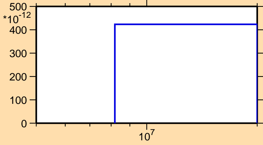
\sigma vs. E for ^{141}\text{Gd}(\text{mt } 34)
