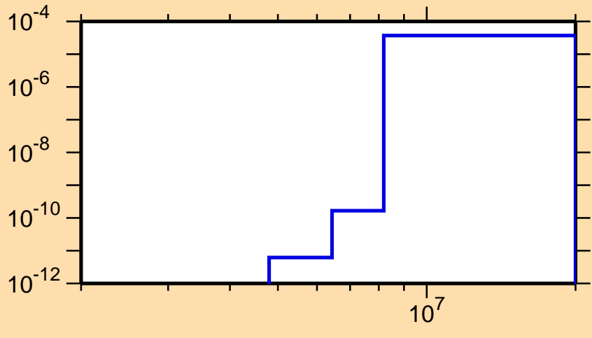
\sigma vs. E for ^{141}\text{Gd}(n,\text{He3})
