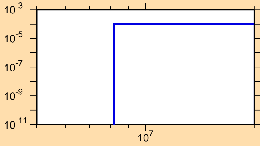
\sigma vs. E for ^{141}\text{Gd}(n,t)
