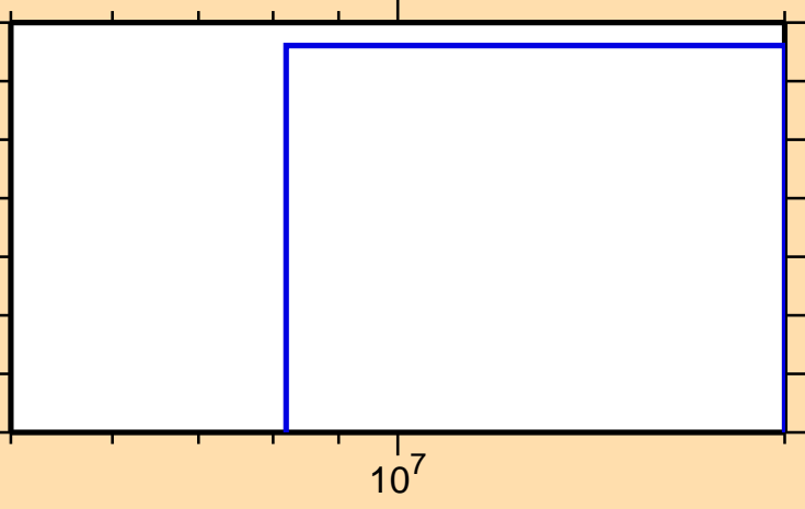
\sigma vs. E for ^{141}\text{Gd}(n,\text{pd})
