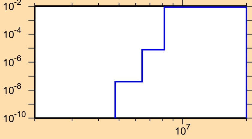
\sigma vs. E for ^{141}\text{Gd}(n,d)
