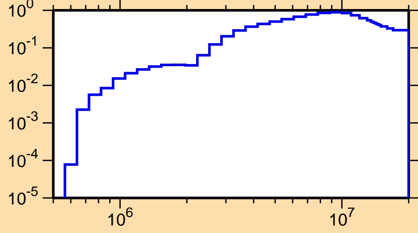
\sigma vs. E for ^{141}\text{Gd}(n,n\text{cont.})
