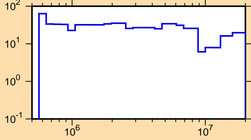
\Delta\sigma/\sigma vs. E for ^{141}\text{Gd}(n,\text{el.})
