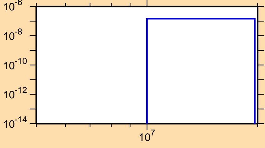
\sigma vs. E for ^{141}\text{Gd}(\text{mt } 45)
