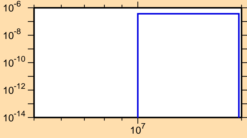
\sigma vs. E for ^{141}\text{Gd}(n,\text{pt})
