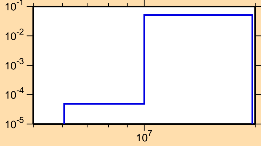
\sigma vs. E for ^{141}\text{Gd}(n,2n)
