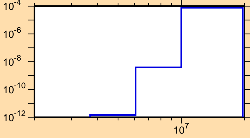
\sigma vs. E for ^{141}\text{Gd}(n,\text{He3})
