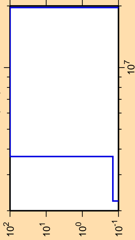
\Delta\sigma/\sigma vs. E for ^{141}\text{Gd}(n,d)
