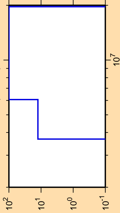
\Delta\sigma/\sigma vs. E for ^{141}\text{Gd}(n,\text{He3})
