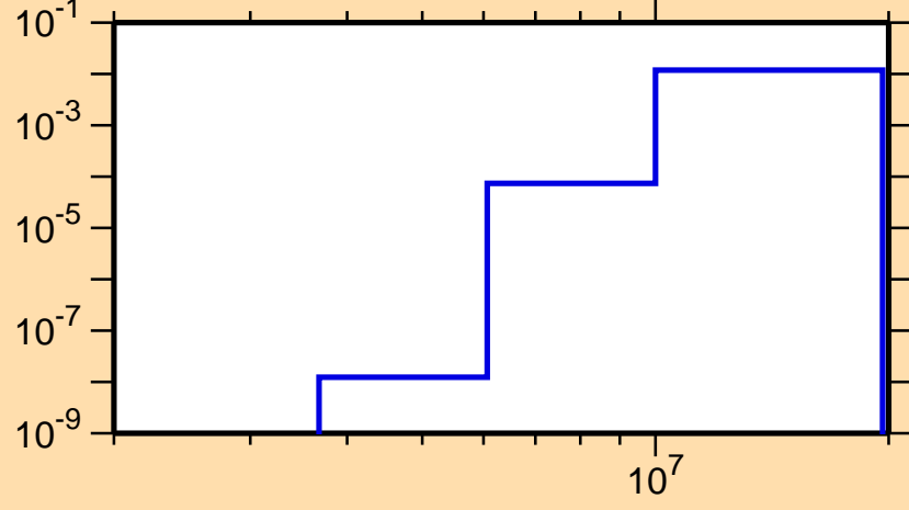
\sigma vs. E for ^{141}\text{Gd}(n,d)
