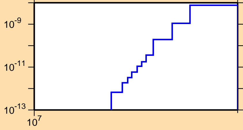
\sigma vs. E for ^{142}\text{Gd}(\text{mt117})
