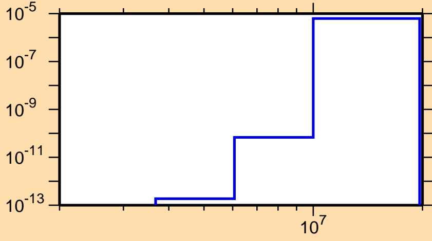
\sigma vs. E for ^{142}\text{Gd}(n,\text{He3})
