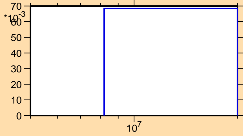
\sigma vs. E for ^{142}\text{Gd}(n,2n)
