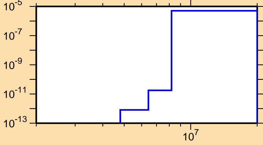
\sigma vs. E for ^{142}\text{Gd}(n,\text{He}3)
