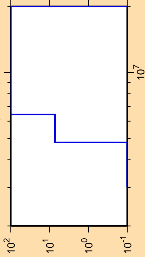
\Delta\sigma/\sigma vs. E for ^{142}\text{Gd}(n,\text{He}3)
