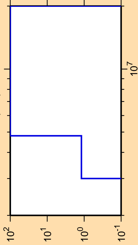
\Delta\sigma/\sigma vs. E for ^{142}\text{Gd}(n,d)
