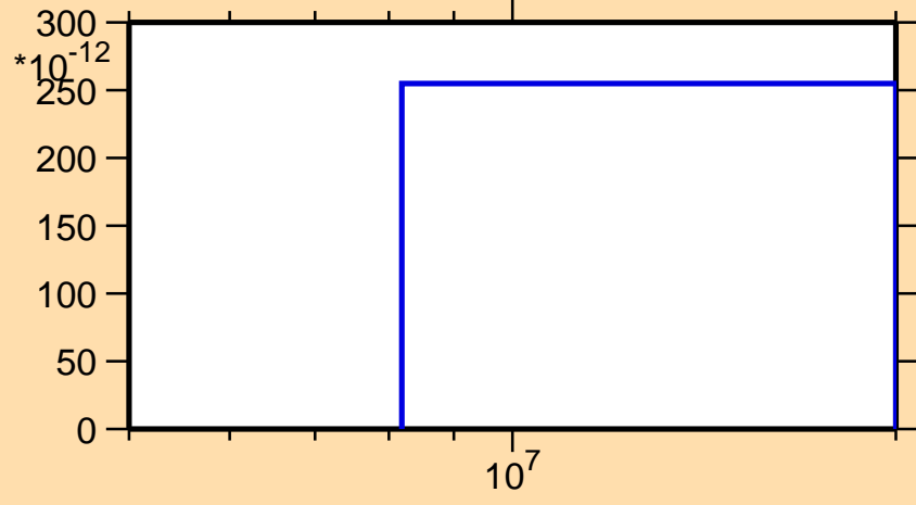
\sigma vs. E for ^{142}\text{Gd}(n,\text{nd})
