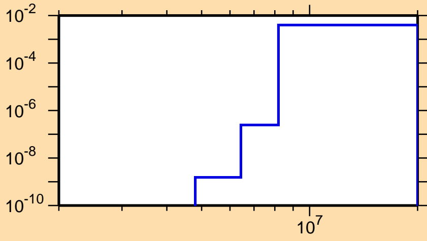
\sigma vs. E for ^{142}\text{Gd}(n,d)
