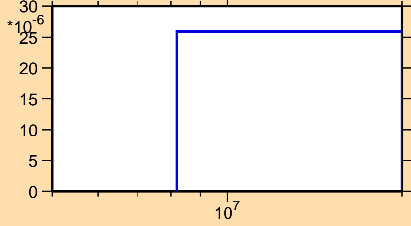
\sigma vs. E for ^{142}\text{Gd}(n,t)
