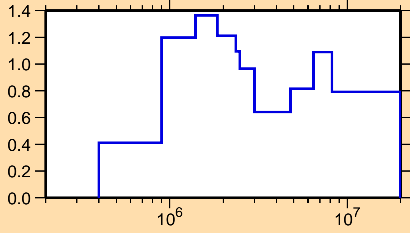
\sigma vs. E for ^{142}\text{Gd}(n,\text{inel.})
