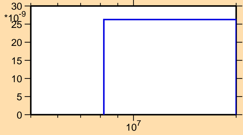
\sigma vs. E for ^{142}\text{Gd}(n,2np)
