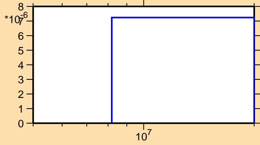
\sigma vs. E for ^{142}\text{Gd}(n,\text{pd})
