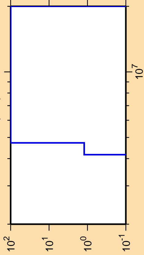
\Delta\sigma/\sigma vs. E for ^{143}\text{Gd}(n,d)
