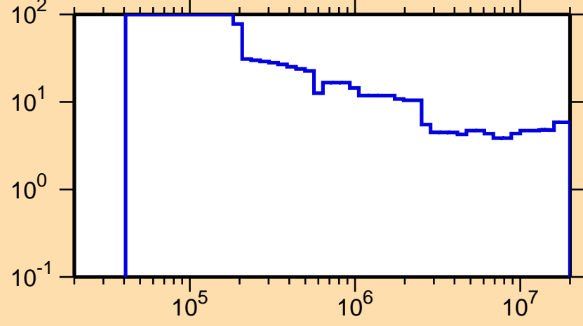
\Delta\sigma/\sigma vs. E for ^{143}\text{Gd}(n,\text{nonel.})
