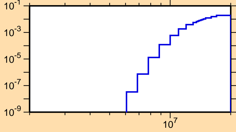
\sigma vs. E for ^{143}\text{Gd}(n,d)
