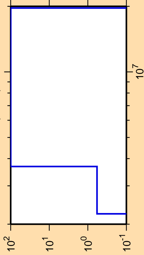
\Delta\sigma/\sigma vs. E for ^{143}\text{Gd}(n,n\alpha)
