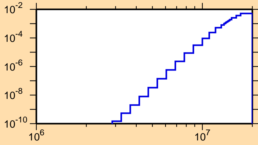
\sigma vs. E for ^{143}\text{Gd}(n,p\alpha)
