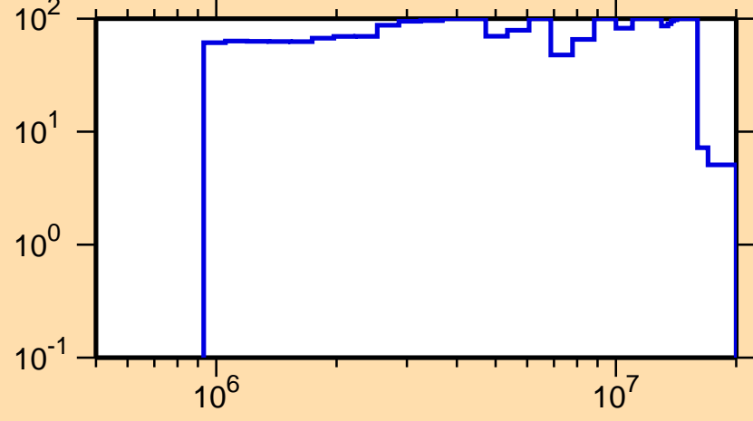
\Delta\sigma/\sigma vs. E for ^{143}\text{Gd}(n,n_1)
