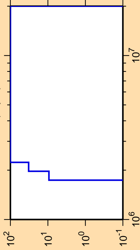
\Delta\sigma/\sigma vs. E for ^{143}\text{Gd}(n,p\alpha)
