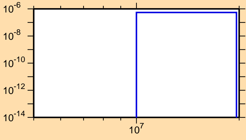
\sigma vs. E for ^{143}\text{Gd}(n,\text{pd})
