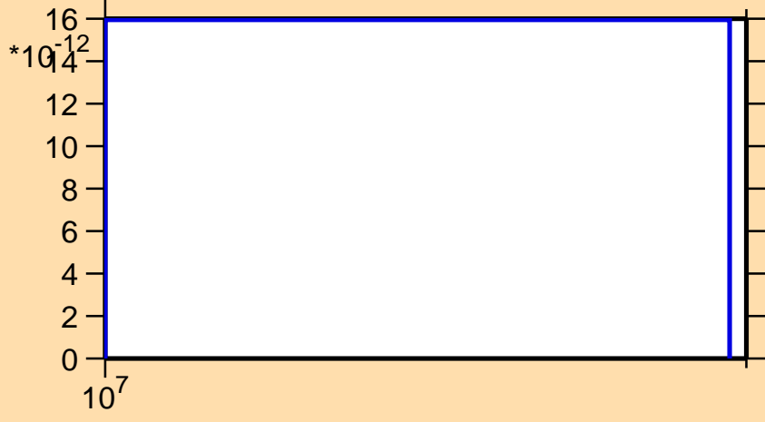
\sigma vs. E for ^{143}\text{Gd} (mt 34)
