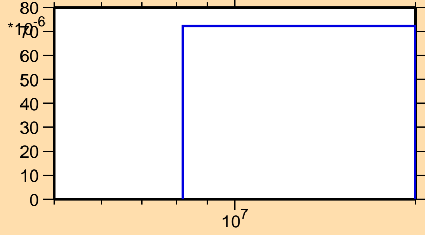
\sigma vs. E for ^{143}\text{Gd}(n,t)
