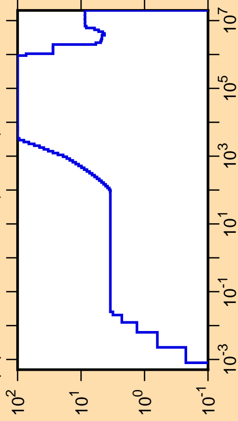
\Delta\mu/\mu vs. E for ^{144}\text{Gd}(\text{mt251})
