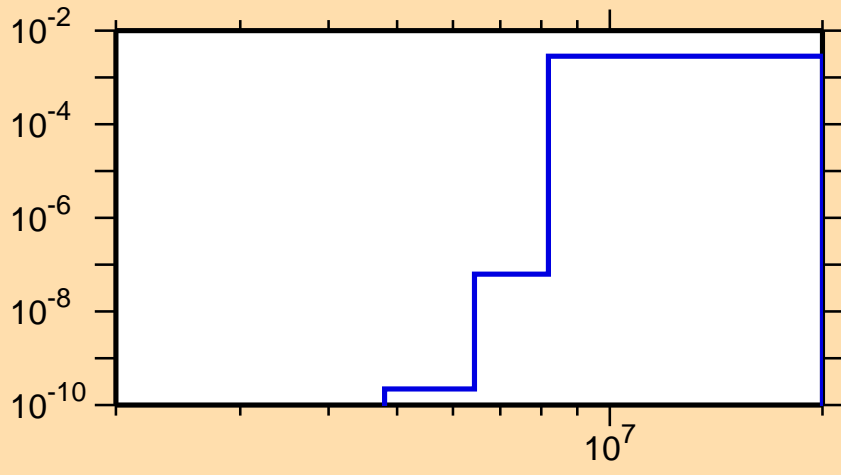
\sigma vs. E for ^{144}\text{Gd}(n,d)
