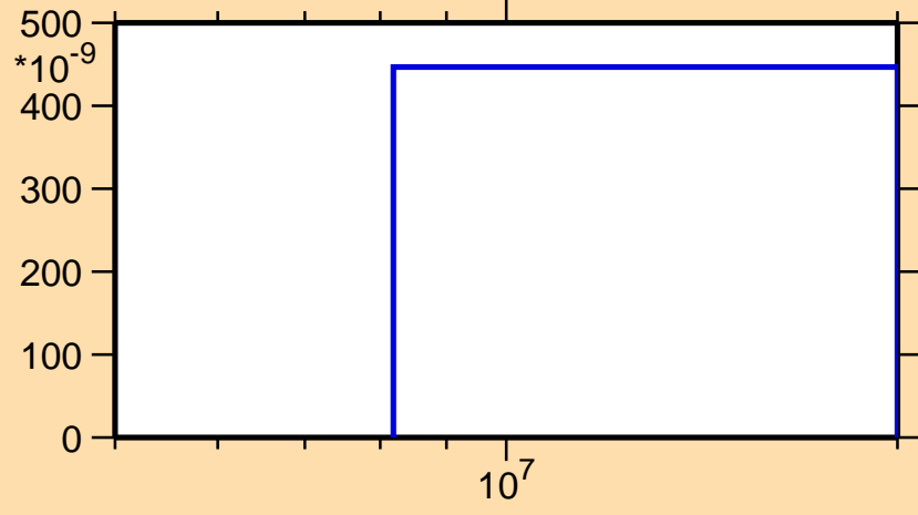
\sigma vs. E for ^{144}\text{Gd}(n,\text{pd})
