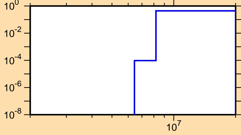
\sigma vs. E for ^{144}\text{Gd}(n,np)
