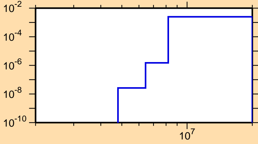
\sigma vs. E for ^{144}\text{Gd}(n,n\alpha)
