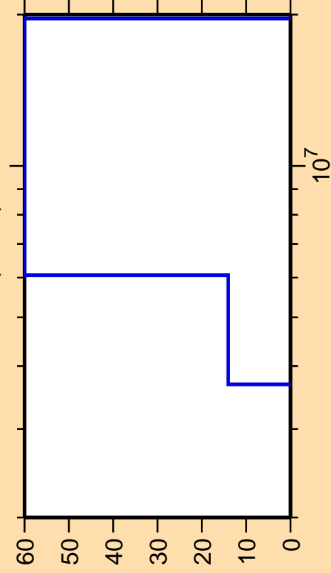
\Delta\sigma/\sigma vs. E for ^{145}\text{Gd}(n,n\alpha)
