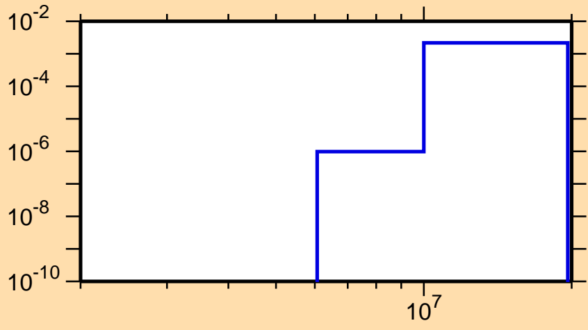
\sigma vs. E for ^{145}\text{Gd}(n,n\alpha)
