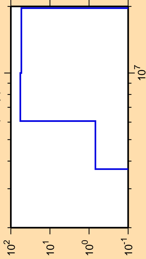
\Delta\sigma/\sigma vs. E for ^{145}\text{Gd}(n,np)
