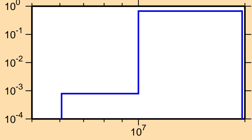
\sigma vs. E for ^{145}\text{Gd}(n,2n)
