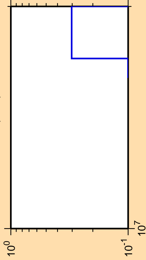
\Delta\sigma/\sigma vs. E for ^{145}\text{Gd}(n,nt)
