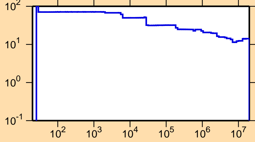
\Delta\sigma/\sigma vs. E for ^{145}\text{Gd}(n,\text{nonel.})
