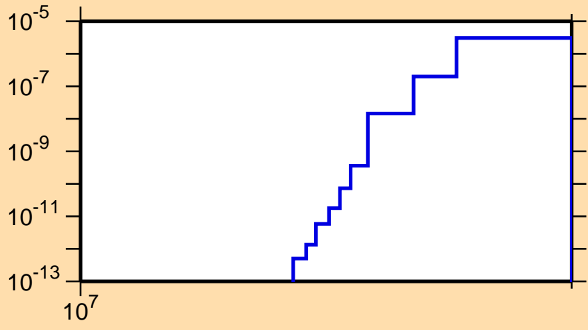
\sigma vs. E for ^{145}\text{Gd}(n,nd)
