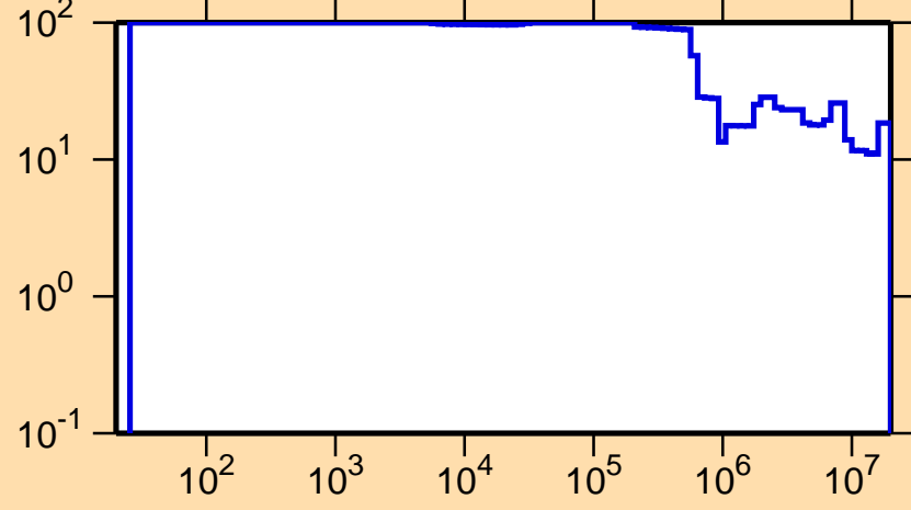
\Delta\sigma/\sigma vs. E for ^{145}\text{Gd}(n,\text{el.})
