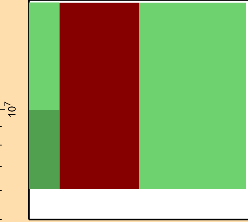
\Delta\sigma/\sigma vs. E for ^{145}\text{Gd}(n,\text{tot.})
