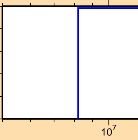
\sigma vs. E for ^{145}\text{Gd}(n,2n\alpha)
