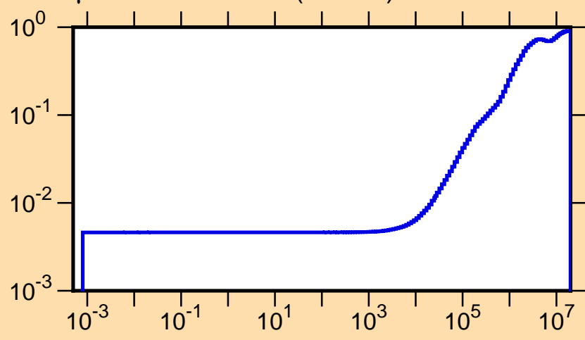
\mu vs. E for ^{146}\text{Gd}(\text{mt251})
