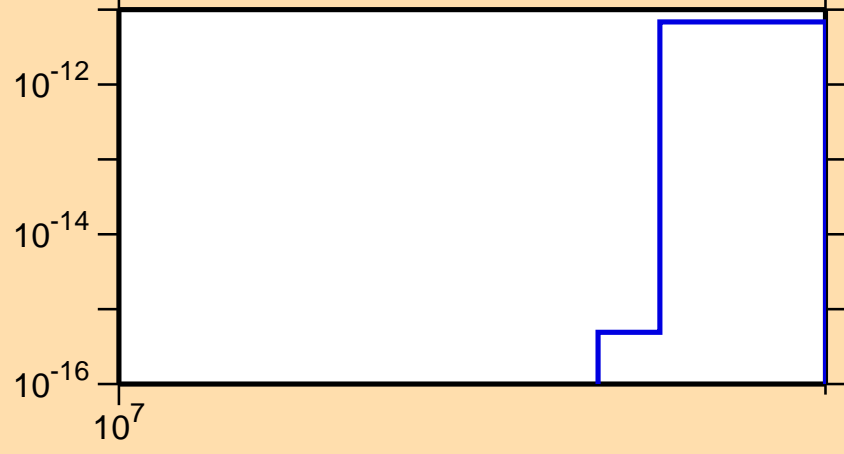
\sigma vs. E for ^{146}\text{Gd}(n,\text{pt})
