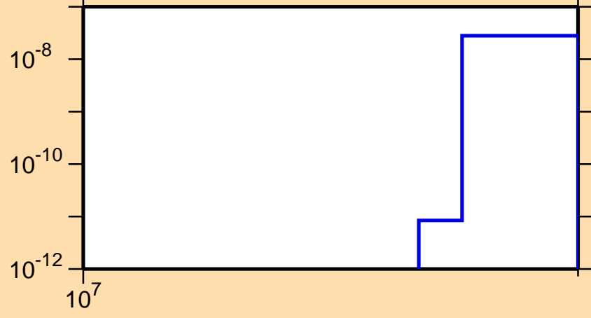
\sigma vs. E for ^{146}\text{Gd}(n,\text{nd})
