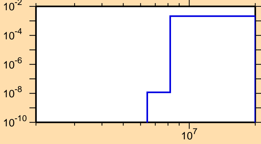
\sigma vs. E for ^{146}\text{Gd}(n,d)
