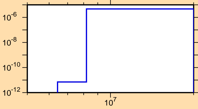
\sigma vs. E for ^{146}\text{Gd}(n,p\alpha)
