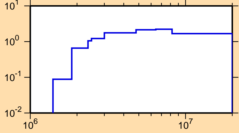
\sigma vs. E for ^{146}\text{Gd}(n,\text{inel.})
