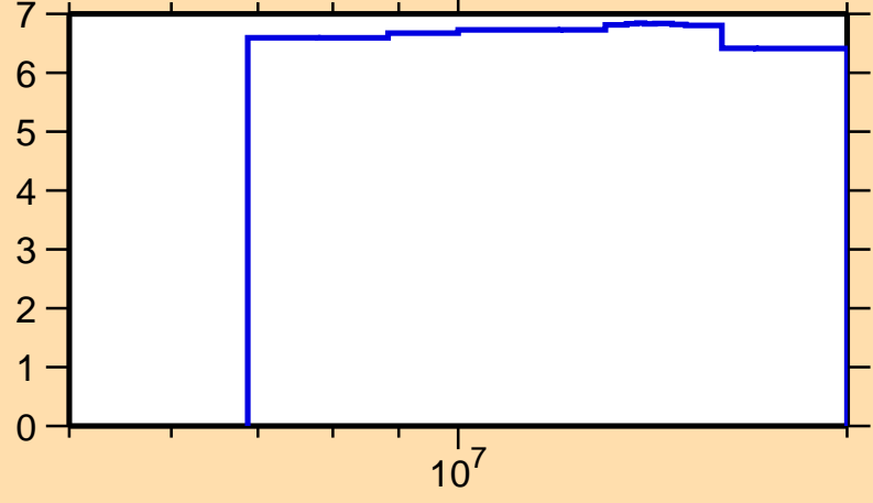
\Delta\sigma/\sigma vs. E for ^{147}\text{Gd}(n,\text{nonel.})
