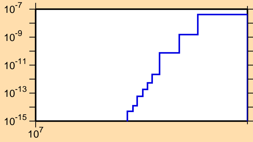
\sigma vs. E for ^{147}\text{Gd}(n,\text{pt})
