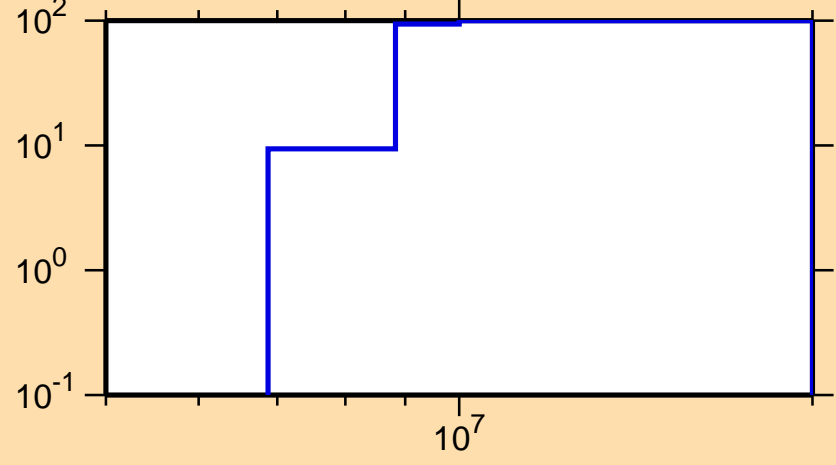
\Delta\sigma/\sigma vs. E for ^{147}\text{Gd}(n,\text{inel.})
