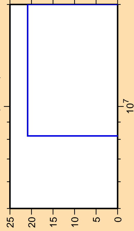
\Delta\sigma/\sigma vs. E for ^{147}\text{Gd}(\text{mt } 34)
