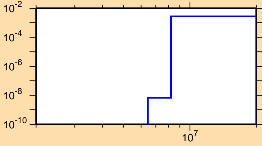
\sigma vs. E for ^{147}\text{Gd}(n,d)
