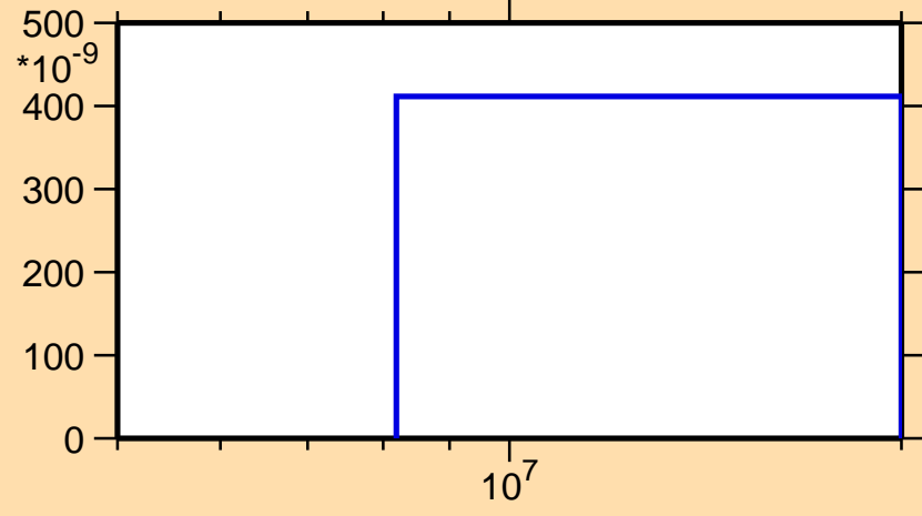
\sigma vs. E for ^{147}\text{Gd}(n,3n)
