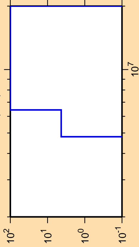
\Delta\sigma/\sigma vs. E for ^{147}\text{Gd}(n,d)
