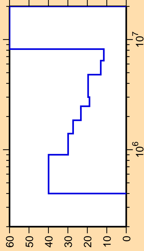
\Delta\sigma/\sigma vs. E for ^{148}\text{Gd}(n,\text{inel.})
