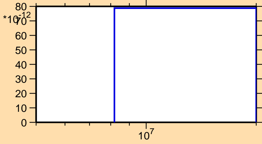
\sigma vs. E for ^{148}\text{Gd}(\text{mt117})
