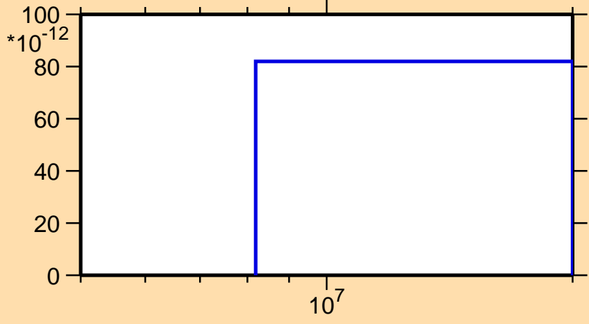
\sigma vs. E for ^{148}\text{Gd}(n,\text{pd})
