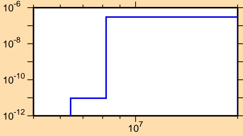
\sigma vs. E for ^{148}\text{Gd}(n,p\alpha)
