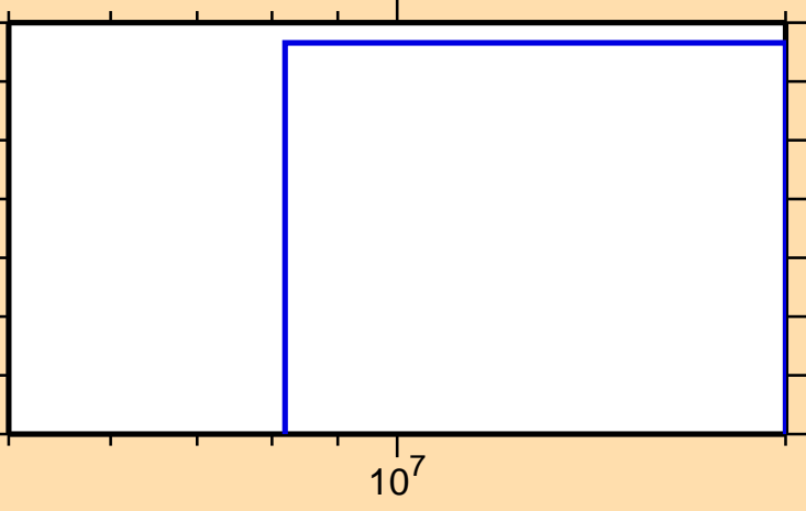
\sigma vs. E for ^{148}\text{Gd}(n,t)
