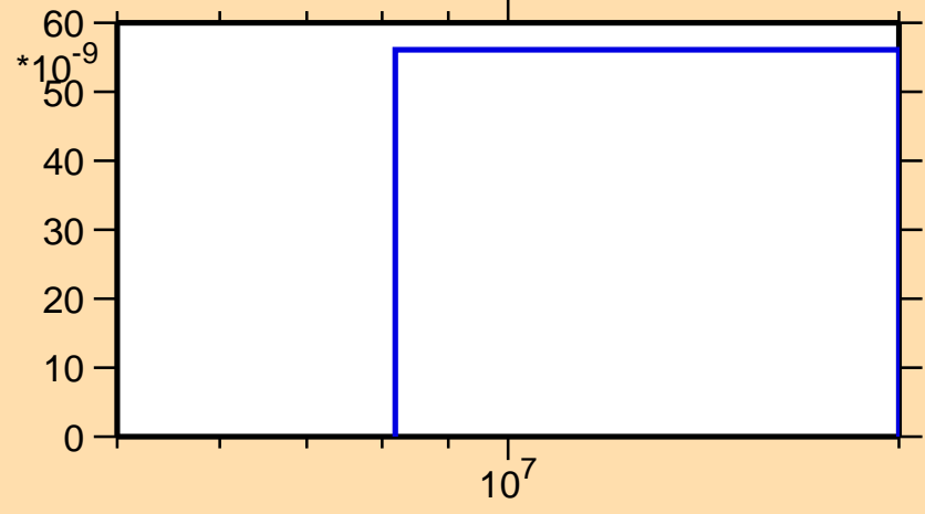
\sigma vs. E for ^{148}\text{Gd}(n,2np)
