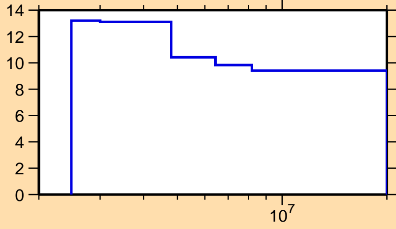
\Delta\sigma/\sigma vs. E for ^{148}\text{Gd}(n,n\text{onel.})
