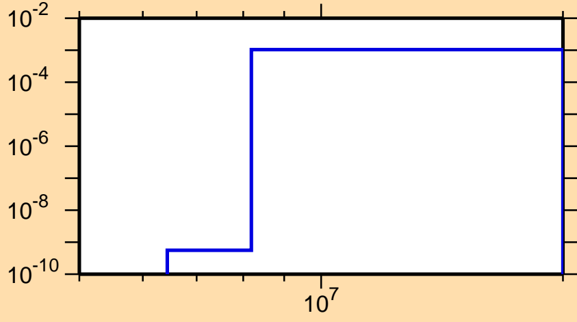
\sigma vs. E for ^{148}\text{Gd}(n,d)
