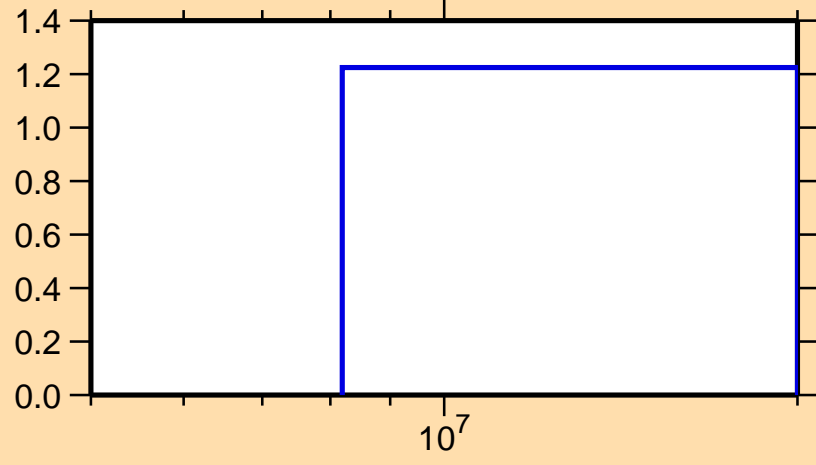
\sigma vs. E for ^{148}\text{Gd}(n,2n)
