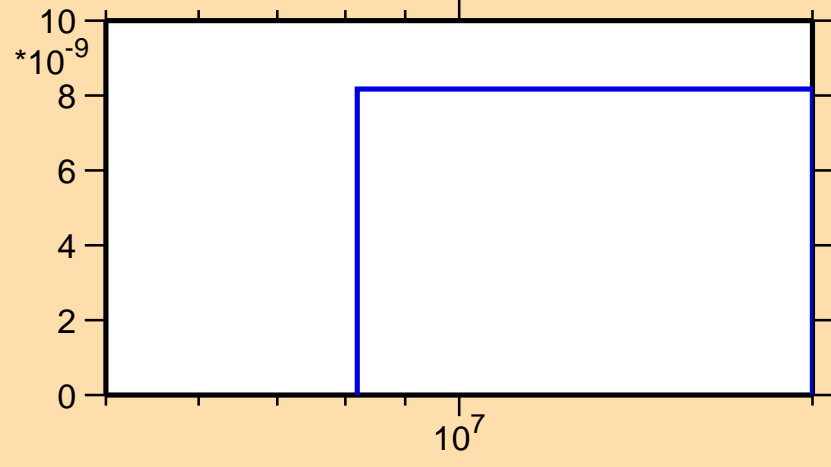
\sigma vs. E for ^{148}\text{Gd}(n,2n\alpha)
