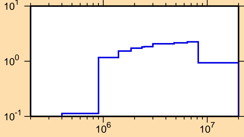
\sigma vs. E for ^{148}\text{Gd}(n,\text{inel.})
