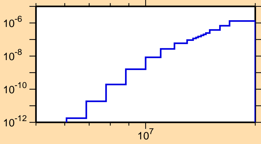
\sigma vs. E for ^{149}\text{Gd}(n,p\alpha)
