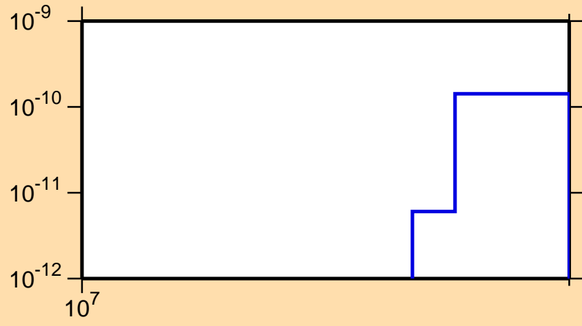
\sigma vs. E for ^{149}\text{Gd}(n,pd)
