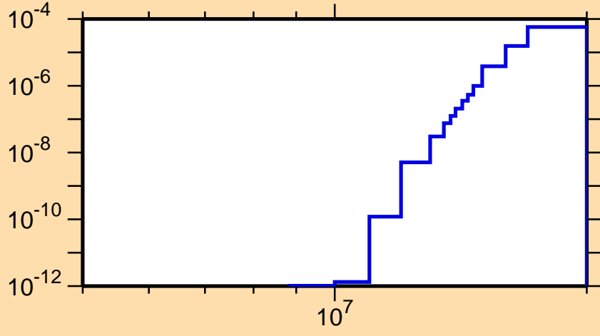
\sigma vs. E for ^{150}\text{Gd}(n,2n\alpha)
