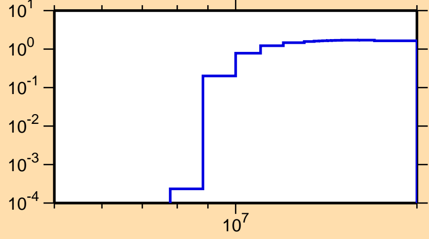
\sigma vs. E for ^{150}\text{Gd}(n,2n)
