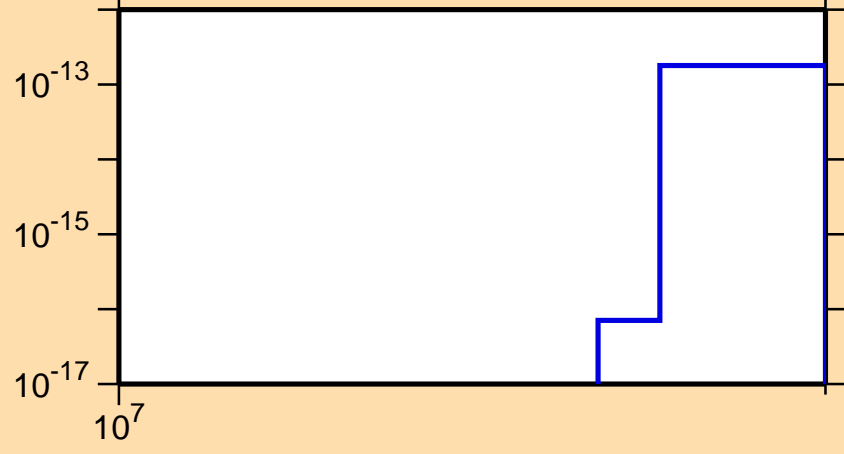
\sigma vs. E for ^{150}\text{Gd}(n,\text{pt})
