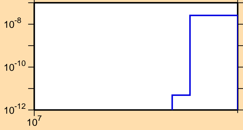
\sigma vs. E for ^{150}\text{Gd}(n,nt)
