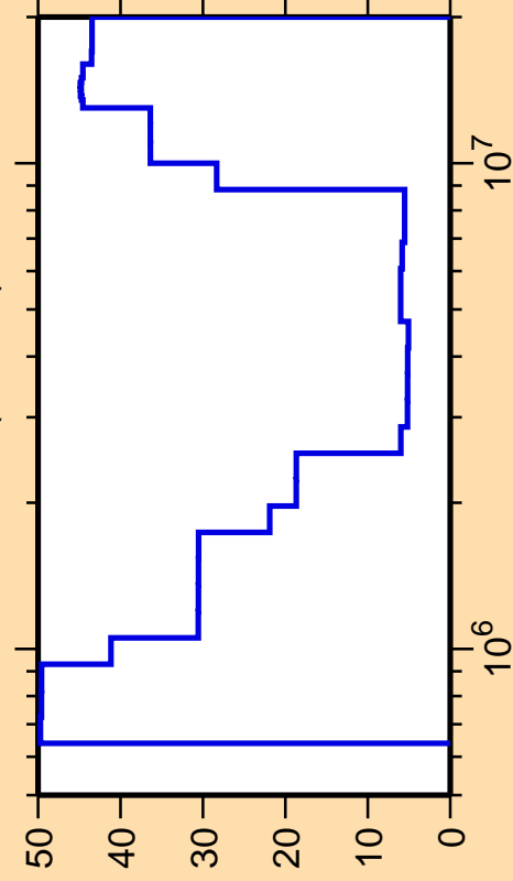
\Delta\sigma/\sigma vs. E for ^{150}\text{Gd}(n,\text{inel.})
