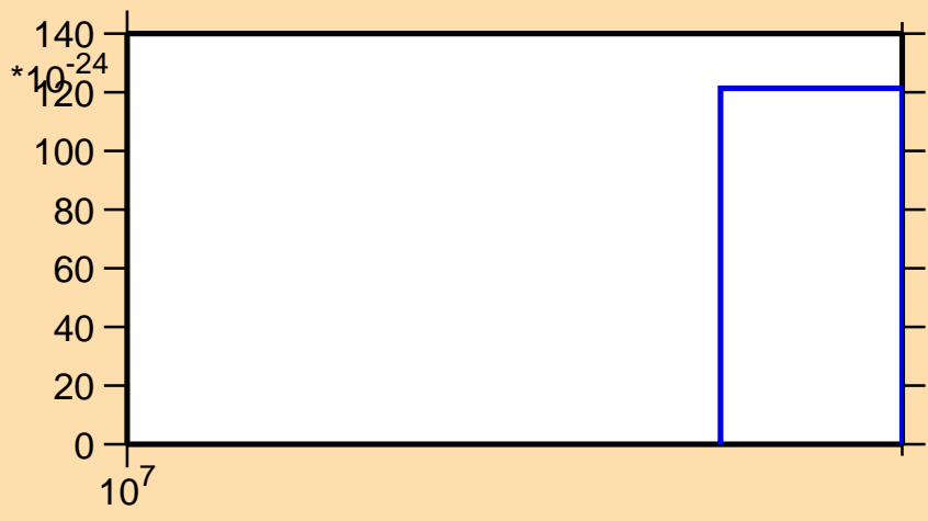
\sigma vs. E for ^{150}\text{Gd}(\text{mt } 11)
