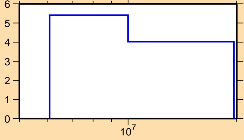
\Delta\sigma/\sigma vs. E for ^{150}\text{Gd}(n,\text{tot.})
