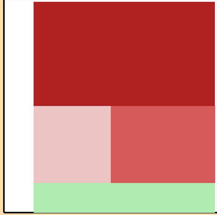
\Delta\sigma/\sigma vs. E for ^{150}\text{Gd}(n,2n)
