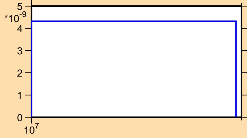
\sigma vs. E for ^{150}\text{Gd}(n,nd)
