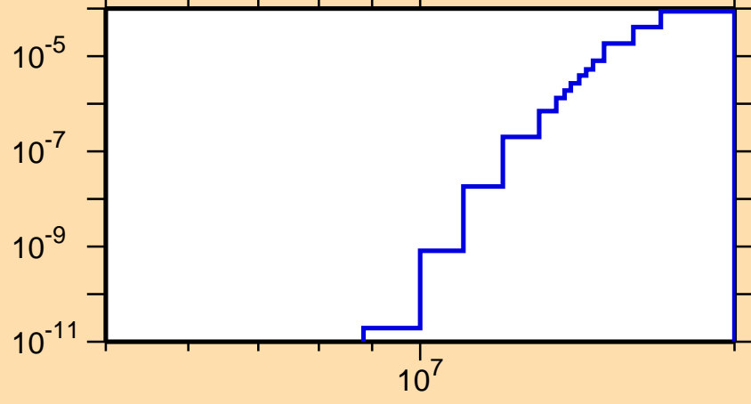
\sigma vs. E for ^{151}\text{Gd}(n,2n\alpha)
