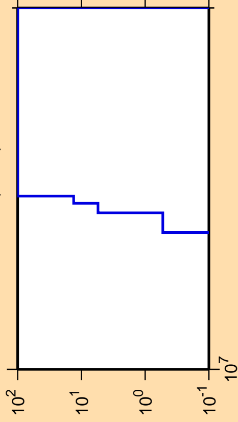
\Delta\sigma/\sigma vs. E for ^{151}\text{Gd}(n,nd)
