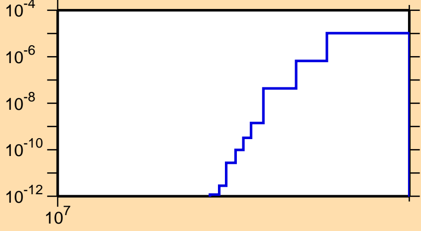
\sigma vs. E for ^{151}\text{Gd}(n,nd)
