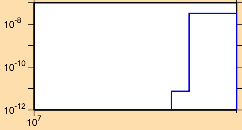
\sigma vs. E for ^{152}\text{Gd}(n,nt)
