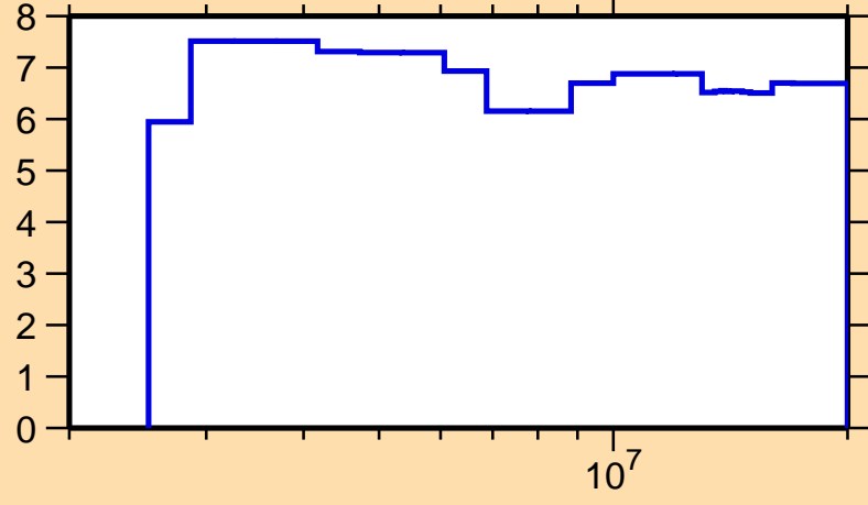
\Delta\sigma/\sigma vs. E for ^{152}\text{Gd}(n,\text{nonel.})
