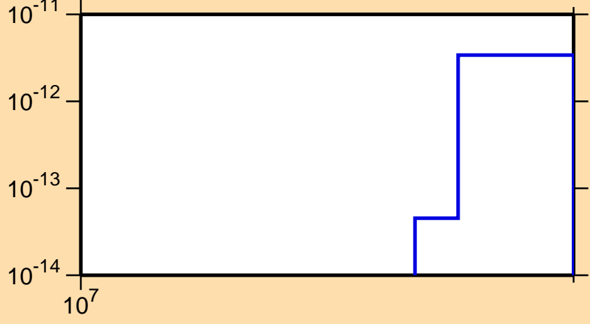
\sigma vs. E for ^{152}\text{Gd} (mt 45)
