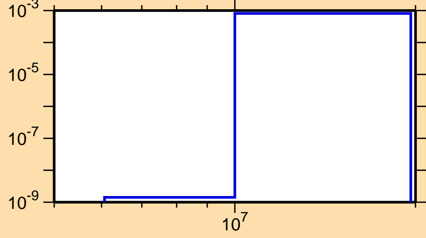
\sigma vs. E for ^{152}\text{Gd}(n,d)
