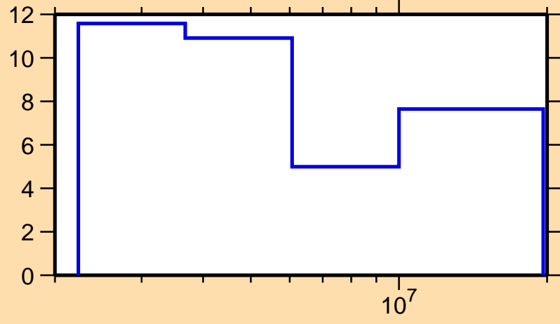
\Delta\sigma/\sigma vs. E for ^{152}\text{Gd}(n,el.)
