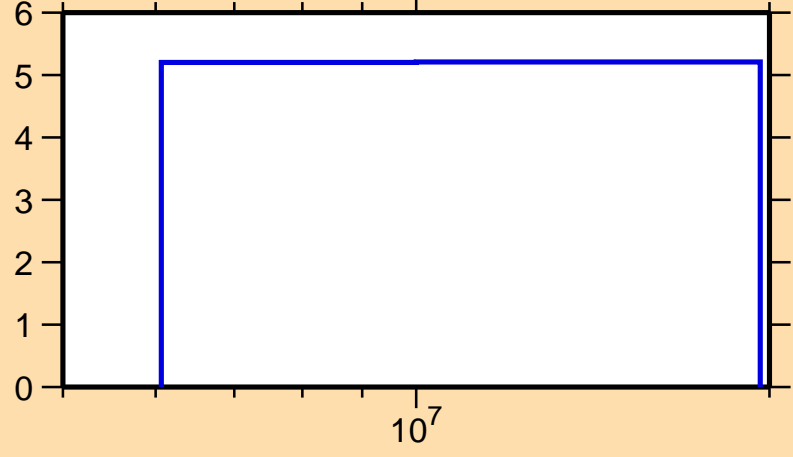
\Delta\sigma/\sigma vs. E for ^{153}\text{Gd}(n,\text{nonel.})
