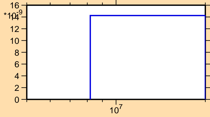
\sigma vs. E for ^{153}\text{Gd}(n,2np)
