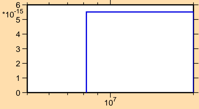
\sigma vs. E for ^{153}\text{Gd}(\text{mt } 34)
