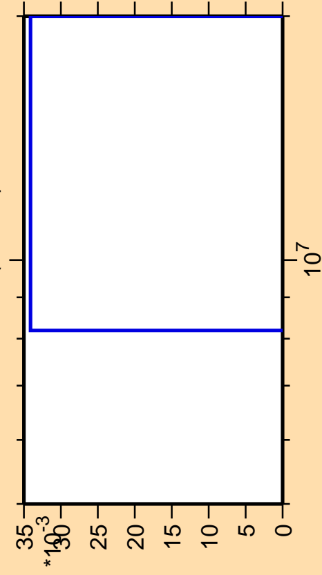
\Delta\sigma/\sigma vs. E for ^{153}\text{Gd}(\text{mt } 34)
