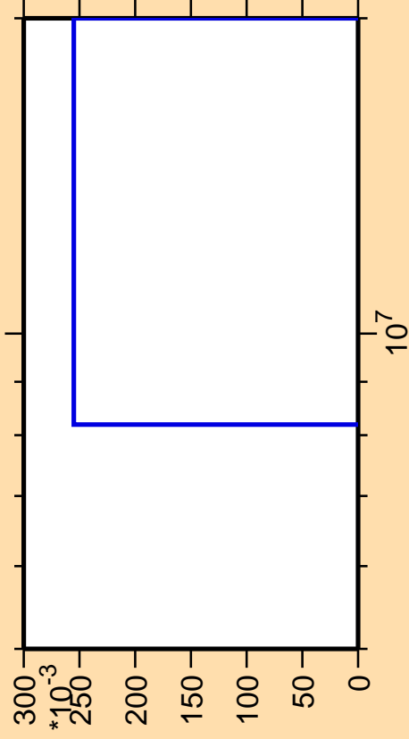
\Delta\sigma/\sigma vs. E for ^{153}\text{Gd}(n,3n\alpha)
