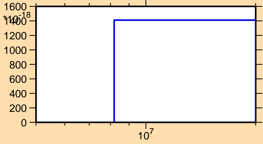
\sigma vs. E for ^{153}\text{Gd}(n,\text{pt})
