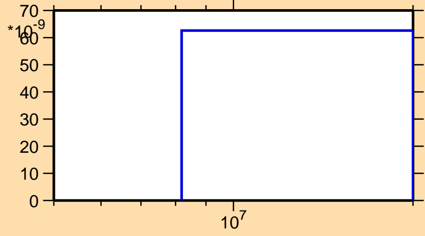
\sigma vs. E for ^{153}\text{Gd}(n,\text{nd})
