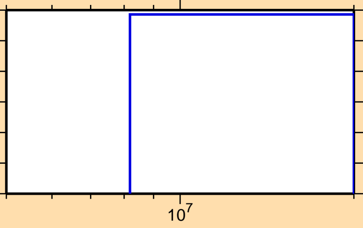
\sigma vs. E for ^{153}\text{Gd}(n,nt)
