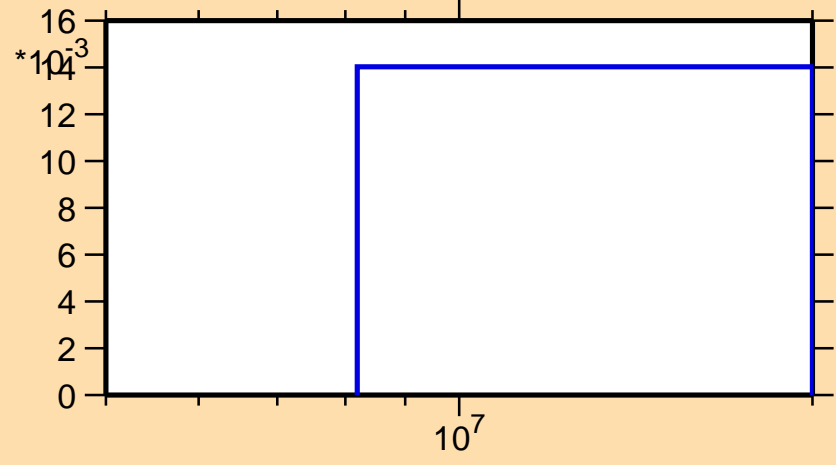
\sigma vs. E for ^{153}\text{Gd}(n,3n)
