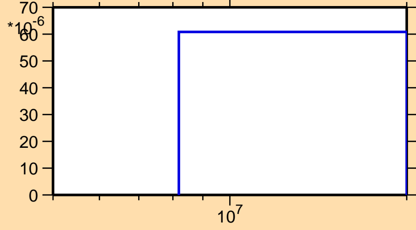
\sigma vs. E for ^{153}\text{Gd}(n,t)
