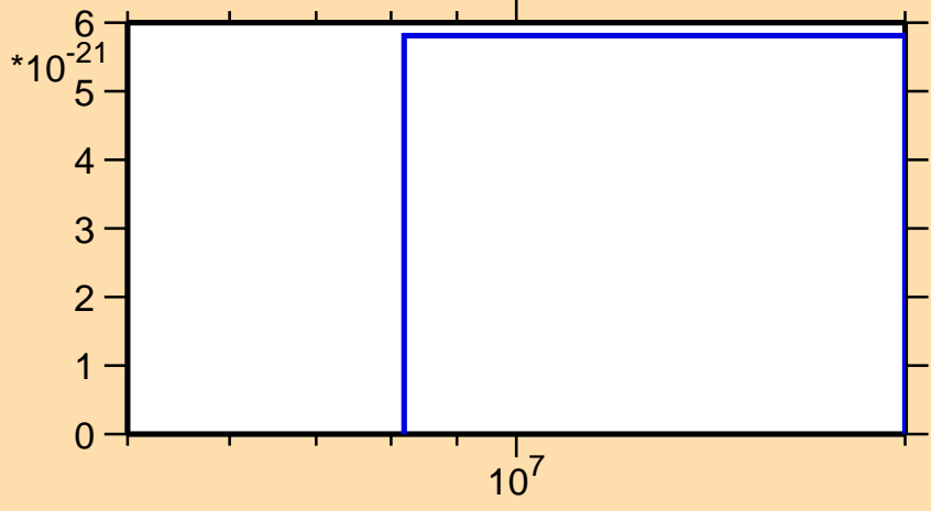
\sigma vs. E for ^{153}\text{Gd}(\text{mt } 11)
