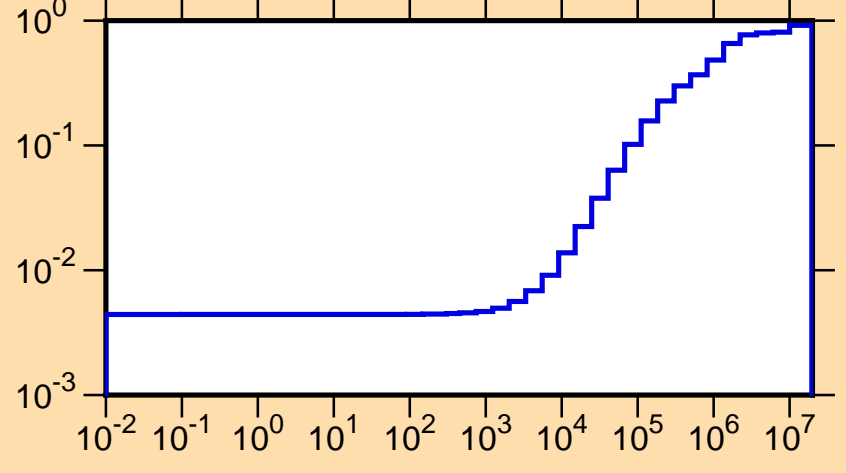
\mu vs. E for ^{154}\text{Gd}(\text{mt251})
