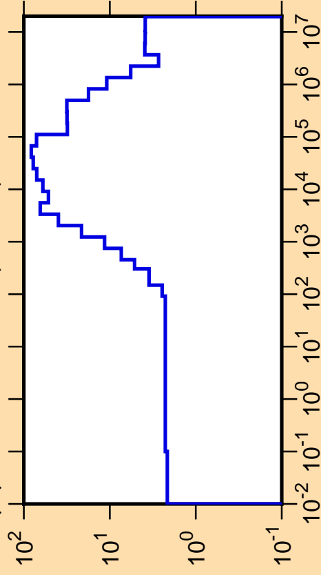
\Delta\mu/\mu vs. E for ^{154}\text{Gd}(\text{mt251})
