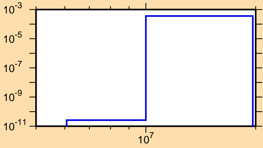
\sigma vs. E for ^{154}\text{Gd}(n,np)
