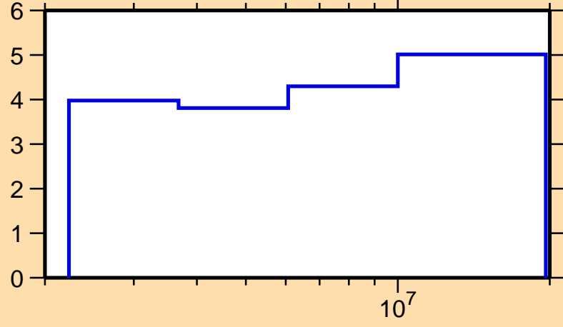
\Delta\sigma/\sigma vs. E for ^{154}\text{Gd}(n,\text{nonel.})
