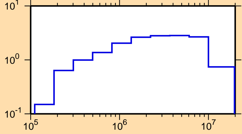
\sigma vs. E for ^{154}\text{Gd}(n,\text{inel.})
