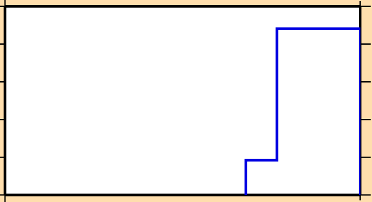
\sigma vs. E for ^{156}\text{Gd}(n,2np)
