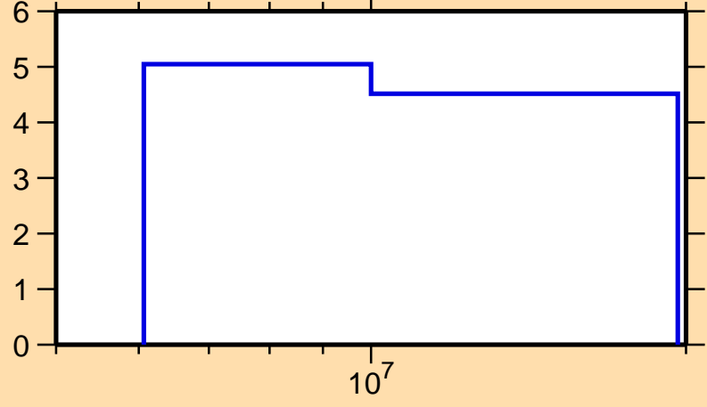
\Delta\sigma/\sigma vs. E for ^{156}\text{Gd}(n,\text{nonel.})
