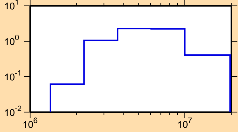
\sigma vs. E for ^{156}\text{Gd}(n,n\text{cont.})
