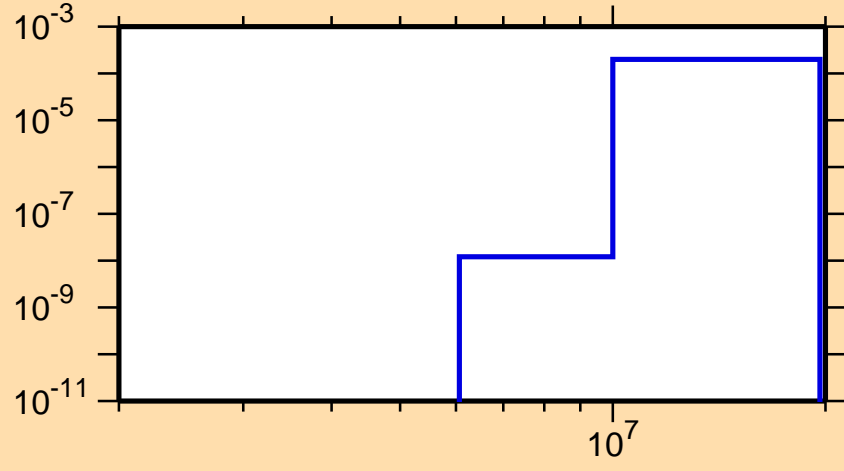
\sigma vs. E for ^{156}\text{Gd}(n,n\alpha)
