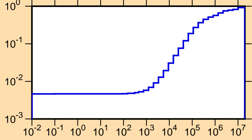
\mu vs. E for ^{157}\text{Gd}(\text{mt251})
