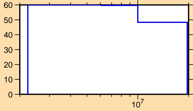
\Delta\sigma/\sigma vs. E for ^{157}\text{Gd}(n,p)
