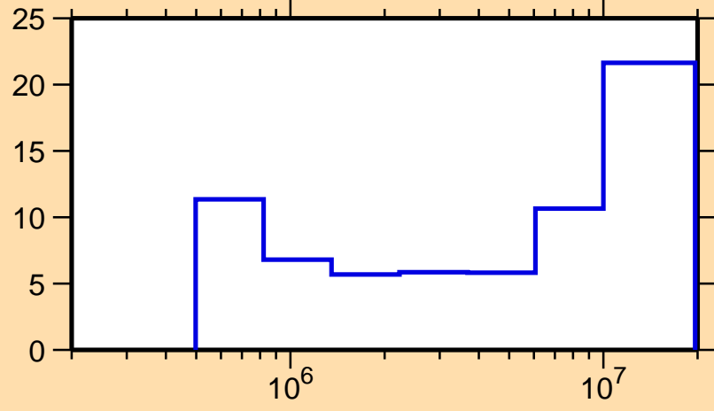
\Delta\sigma/\sigma vs. E for ^{157}\text{Gd}(n,inel.)
