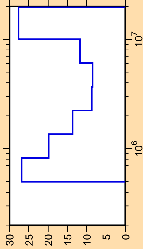
\Delta\sigma/\sigma vs. E for ^{157}\text{Gd}(n,ncont.)
