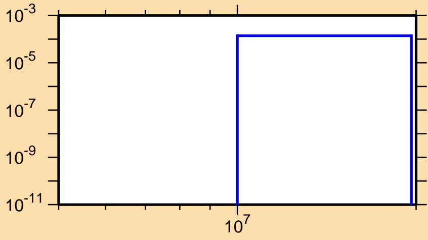
\sigma vs. E for ^{157}\text{Gd}(n,np)
