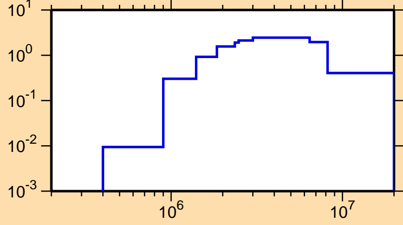
\sigma vs. E for ^{157}\text{Gd}(n,n\text{cont.})
