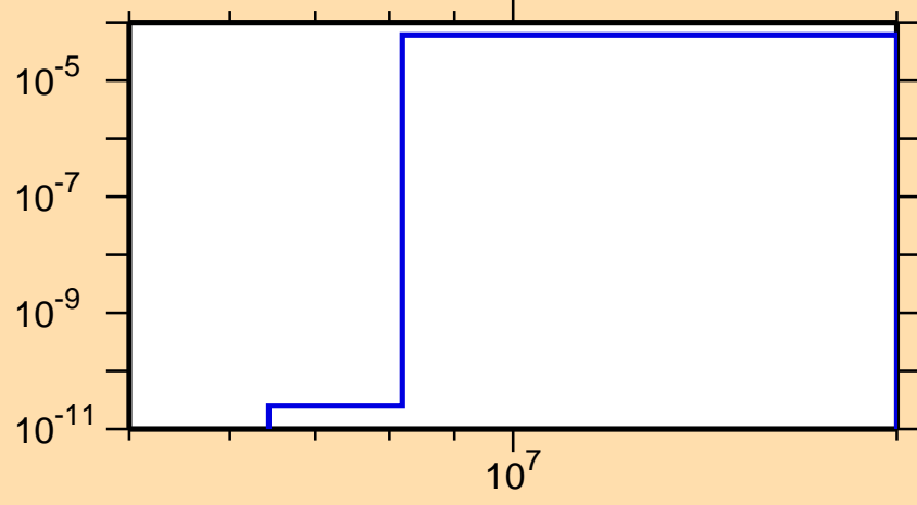
\sigma vs. E for ^{157}\text{Gd}(n,n\alpha)
