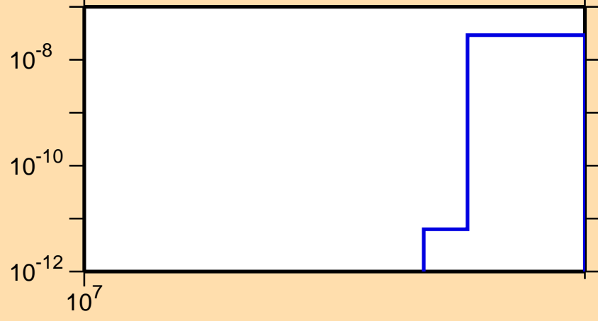
\sigma vs. E for ^{158}\text{Gd}(n,\text{nd})
