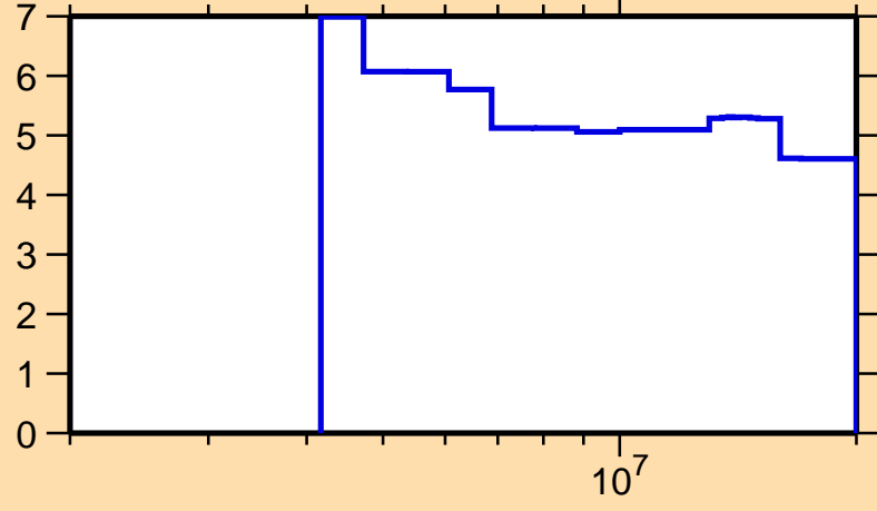
\Delta\sigma/\sigma vs. E for ^{158}\text{Gd}(n,\text{nonel.})
