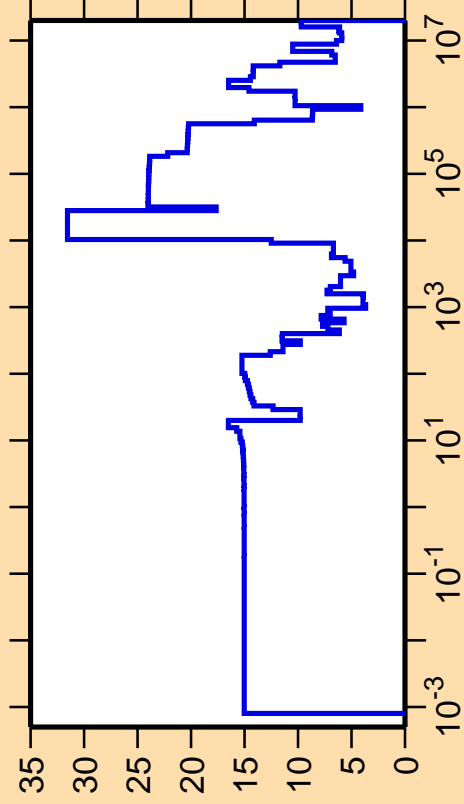
\Delta\sigma/\sigma vs. E for ^{158}\text{Gd}(n,\text{el.})
