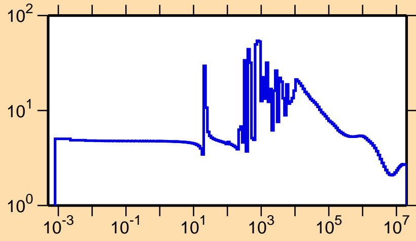
\sigma vs. E for ^{158}\text{Gd}(n,\text{el.})
