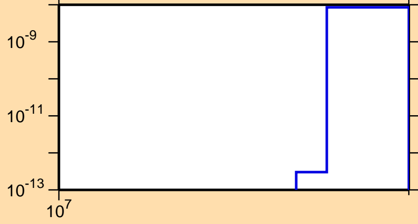
\sigma vs. E for ^{158}\text{Gd}(n,nt)
