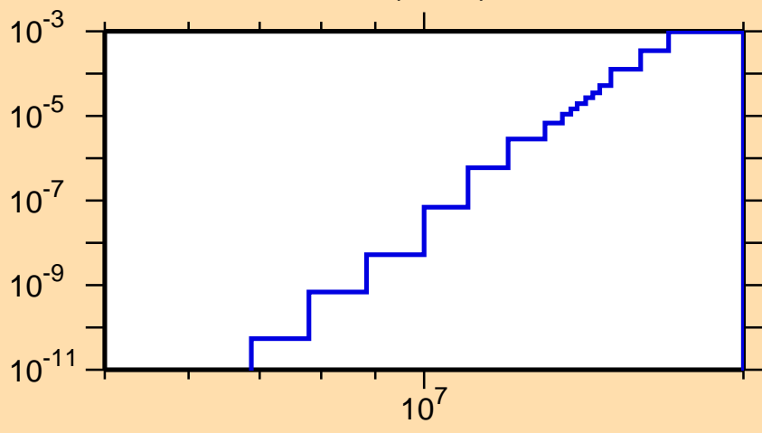
\sigma vs. E for ^{158}\text{Gd}(n,n\alpha)
