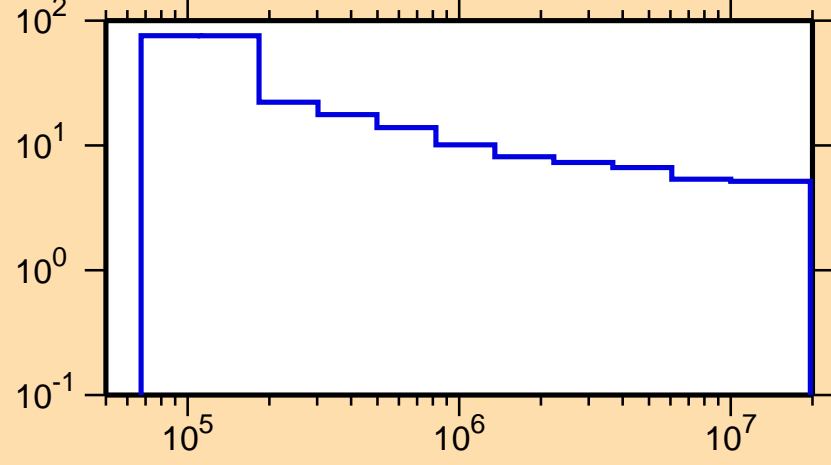
\Delta\sigma/\sigma vs. E for ^{158}\text{Gd}(n,\text{nonel.})
