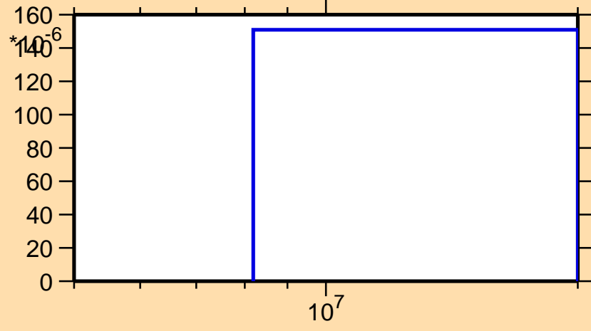
\sigma vs. E for ^{158}\text{Gd}(n,d)
