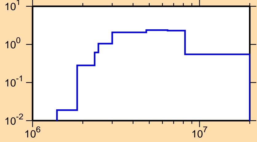
\sigma vs. E for ^{158}\text{Gd}(n,n\text{cont.})
