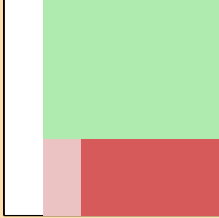
\Delta\sigma/\sigma vs. E for ^{158}\text{Gd}(n,2n)
