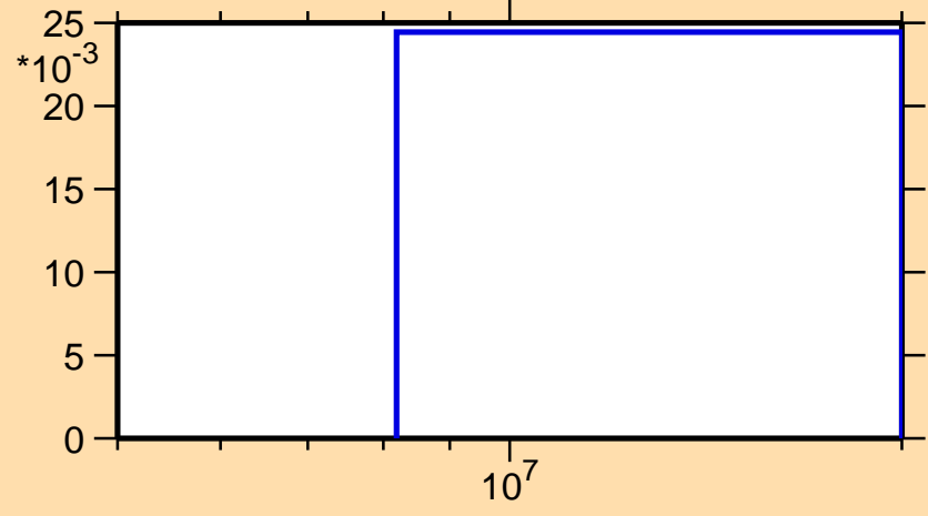
\sigma vs. E for ^{158}\text{Gd}(n,3n)
