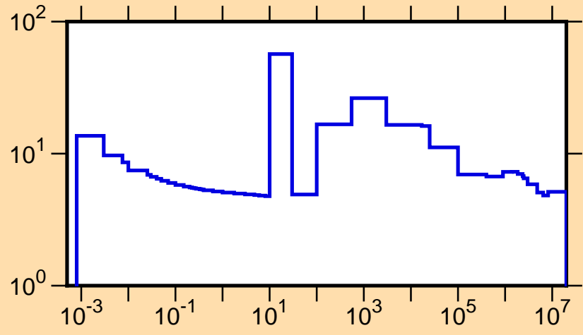
\sigma vs. E for ^{158}\text{Gd}(n,\text{tot.})
