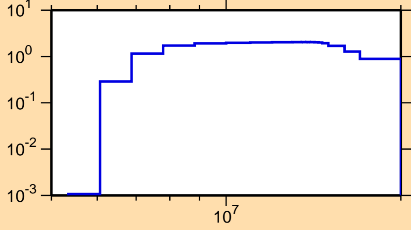
\sigma vs. E for ^{159}\text{Gd}(n,2n)
