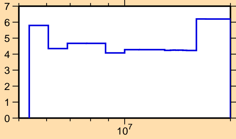
\Delta\sigma/\sigma vs. E for ^{159}\text{Gd}(n,\text{tot.})
