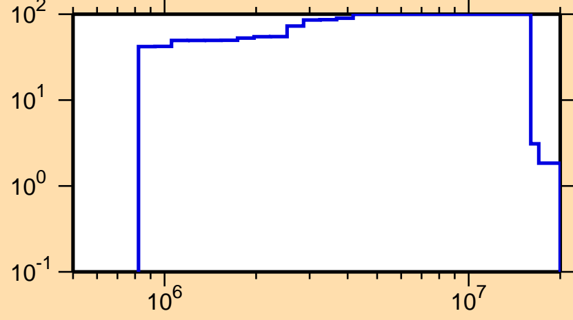
\Delta\sigma/\sigma vs. E for ^{159}\text{Gd}(n,n_1)
