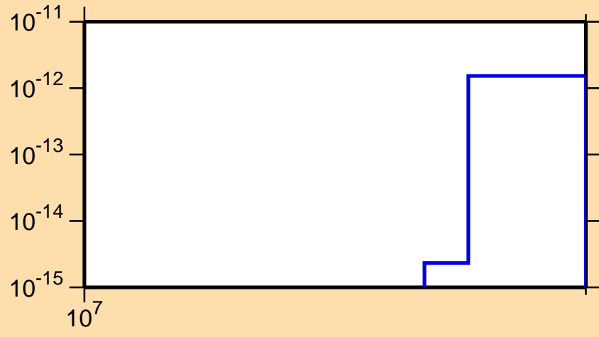
\sigma vs. E for ^{159}\text{Gd}(n,\text{He}3)
