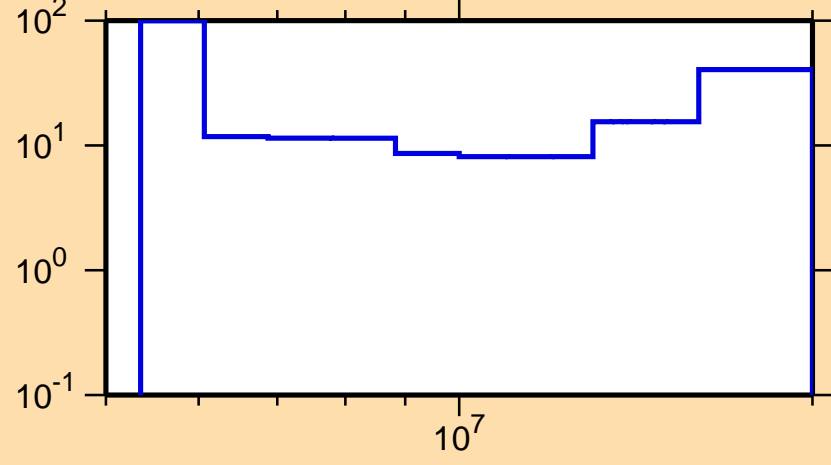
\Delta\sigma/\sigma vs. E for ^{159}\text{Gd}(n,2n)
