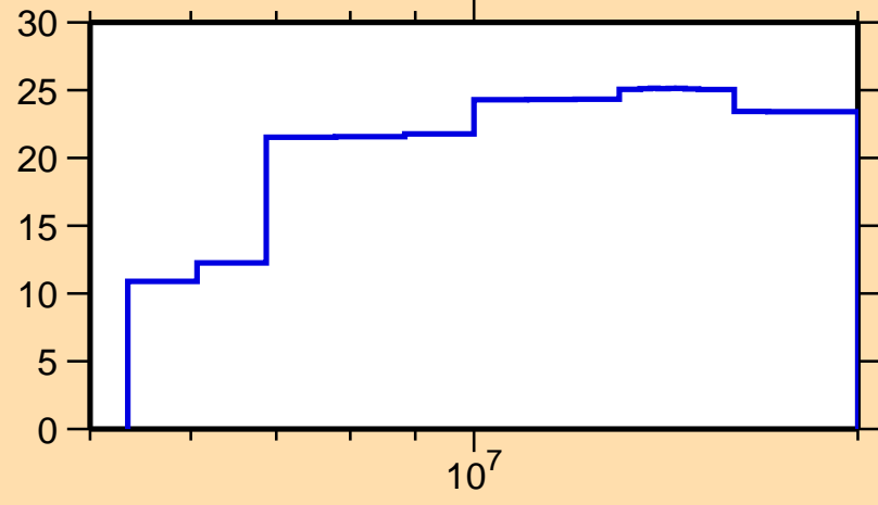
\Delta\sigma/\sigma vs. E for ^{159}\text{Gd}(n,\text{inel.})
