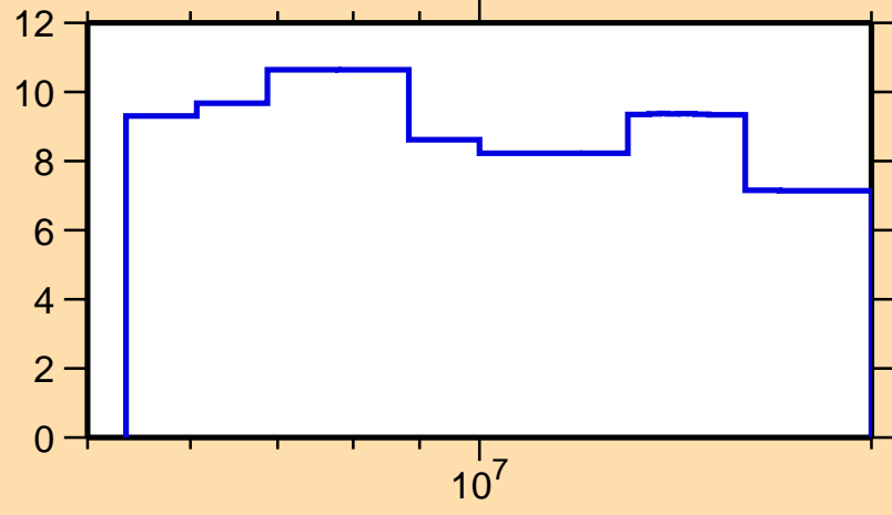
\Delta\sigma/\sigma vs. E for ^{159}\text{Gd}(n,\text{nonel.})
