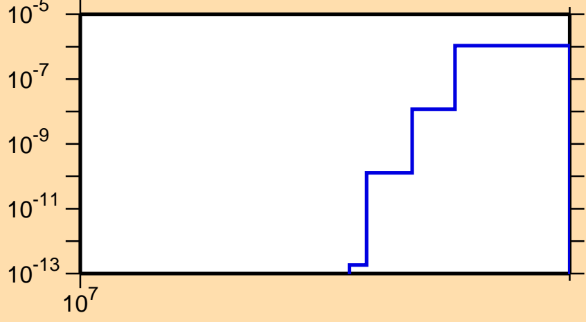
\sigma vs. E for ^{159}\text{Gd}(n,\text{nd})
