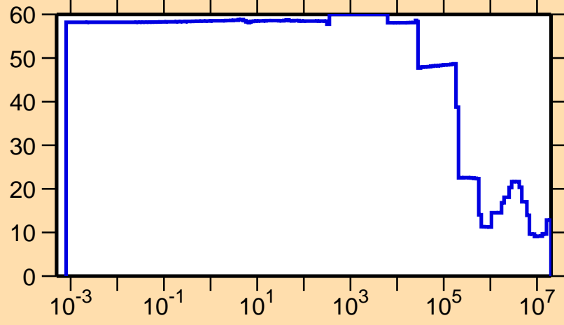
\Delta\sigma/\sigma vs. E for ^{159}\text{Gd}(n,\text{el.})
