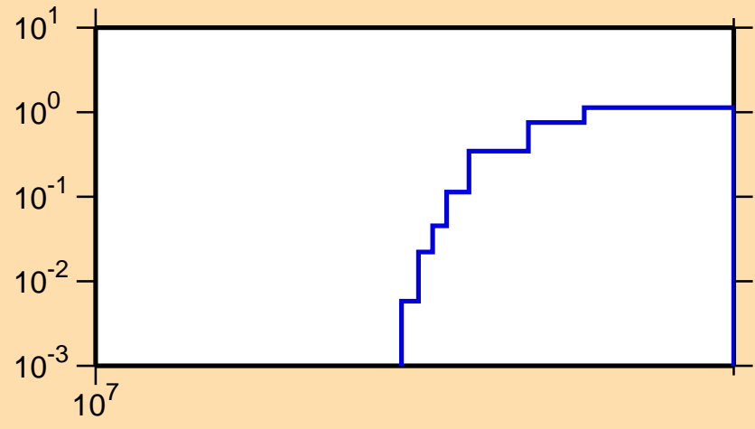
\sigma vs. E for ^{159}\text{Gd}(n,3n)
