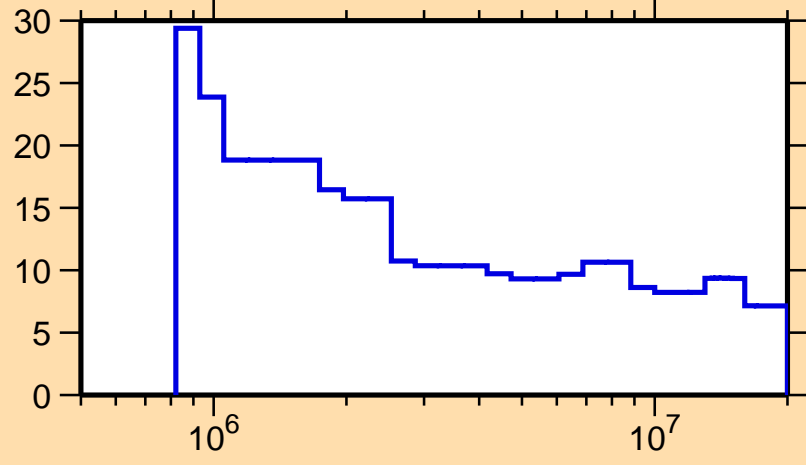
\Delta\sigma/\sigma vs. E for ^{159}\text{Gd}(n,n\text{onel.})
