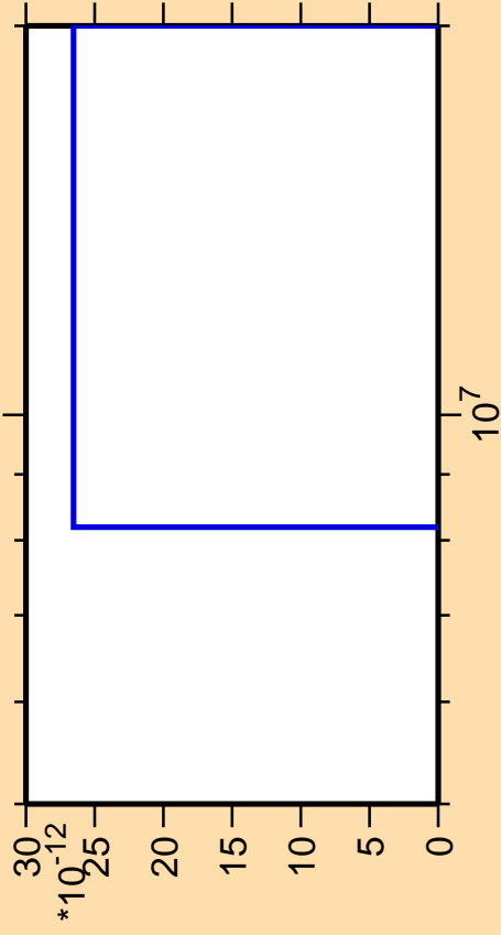
\Delta\sigma/\sigma vs. E for ^{159}\text{Gd}(\text{mt } 11)
