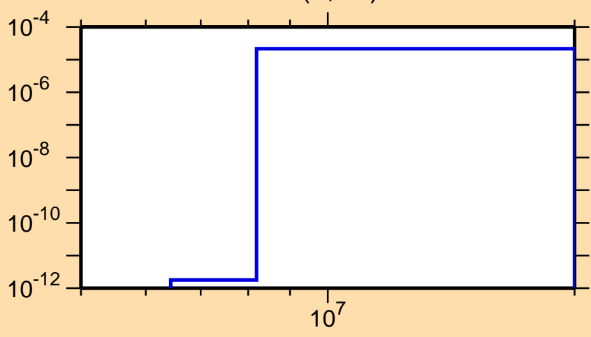
\sigma vs. E for ^{159}\text{Gd}(n,n\alpha)
