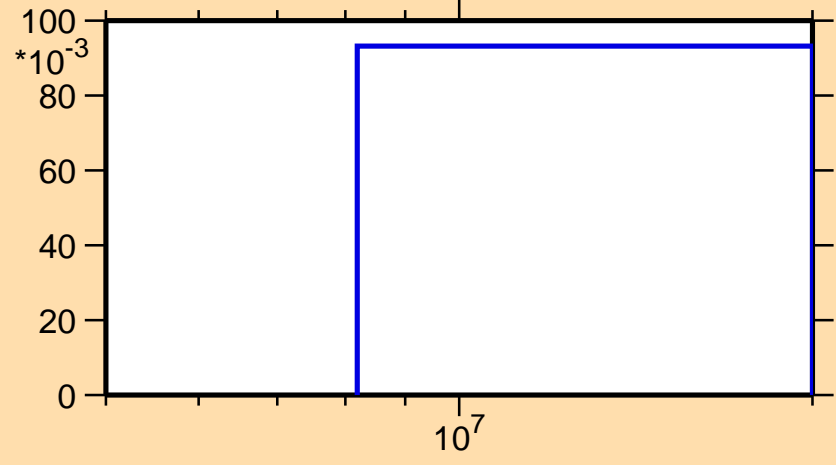
\sigma vs. E for ^{159}\text{Gd}(n,3n)
