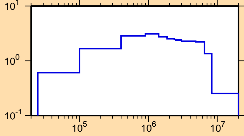
\sigma vs. E for ^{159}\text{Gd}(n,\text{inel.})
