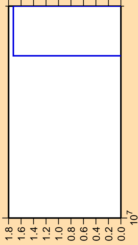
\Delta\sigma/\sigma vs. E for ^{160}\text{Gd}(n,\text{He}3)
