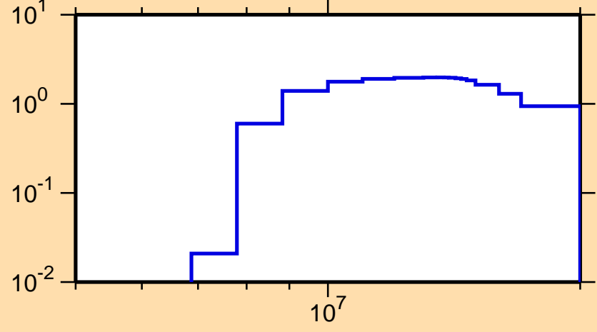
\sigma vs. E for ^{160}\text{Gd}(n,2n)
