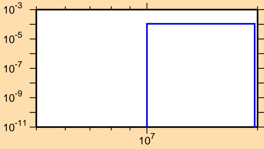
\sigma vs. E for ^{160}\text{Gd}(n,d)
