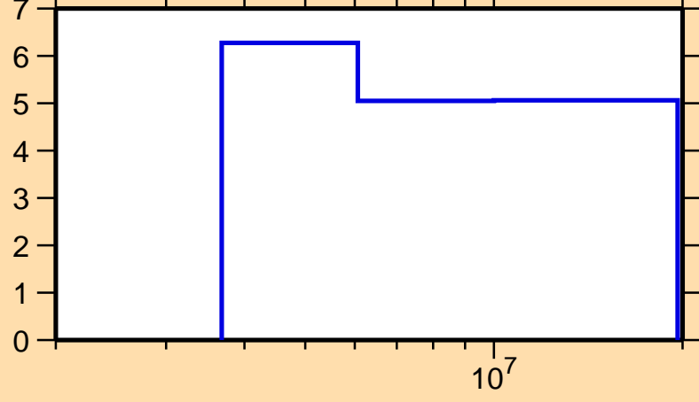
\Delta\sigma/\sigma vs. E for ^{160}\text{Gd}(n,\text{nonel.})
