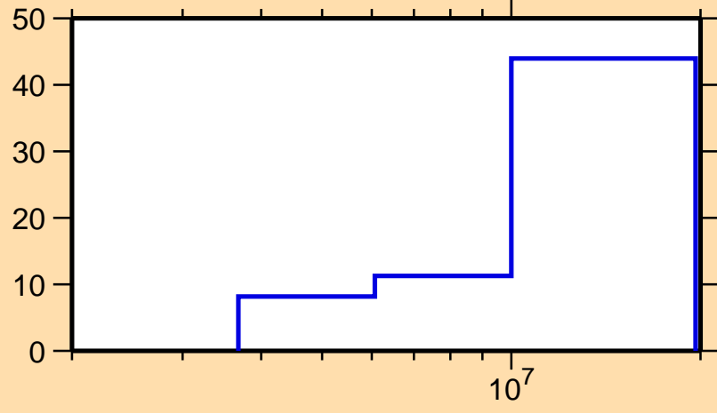
\Delta\sigma/\sigma vs. E for ^{160}\text{Gd}(n,ncont.)
