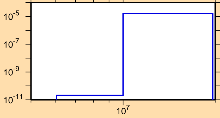
\sigma vs. E for ^{160}\text{Gd}(n,n\alpha)
