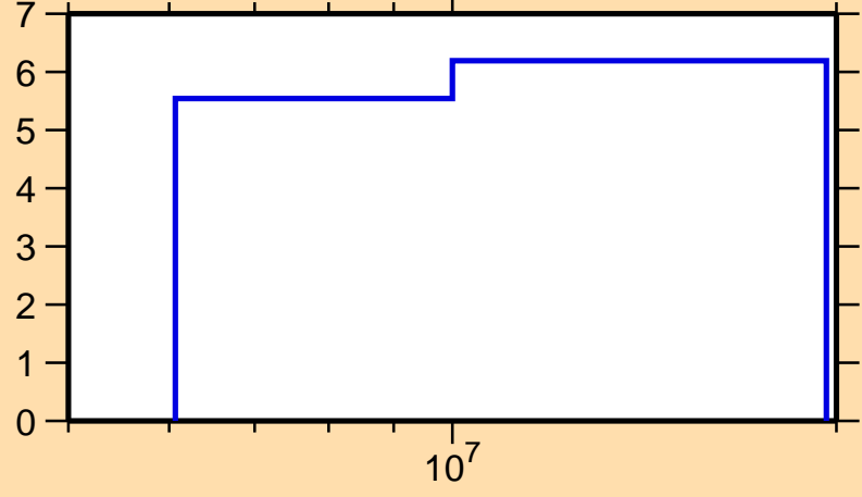
\Delta\sigma/\sigma vs. E for ^{160}\text{Gd}(n,\text{el.})
