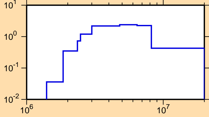
\sigma vs. E for ^{160}\text{Gd}(n,n\text{cont.})
