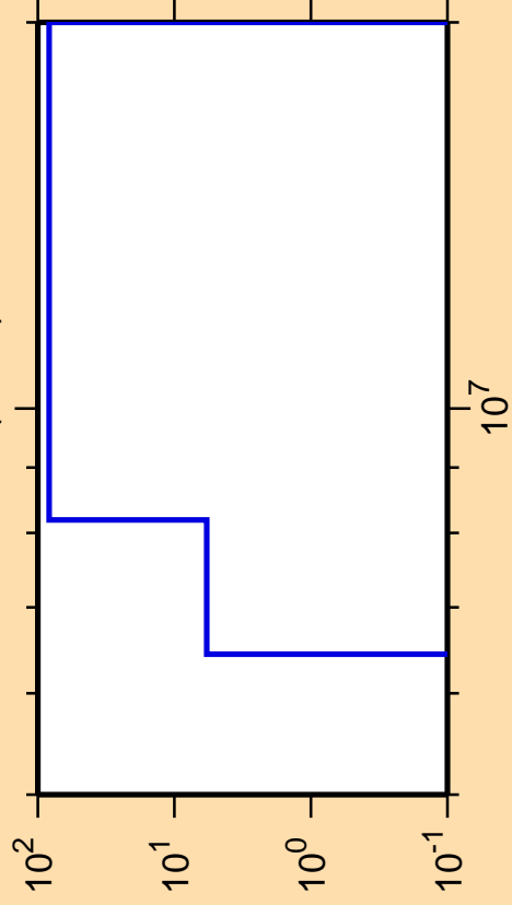
\Delta\sigma/\sigma vs. E for ^{160}\text{Gd}(n,n\alpha)
