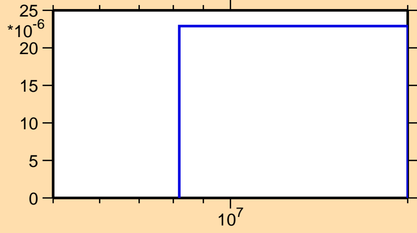
\sigma vs. E for ^{160}\text{Gd}(n,np)
