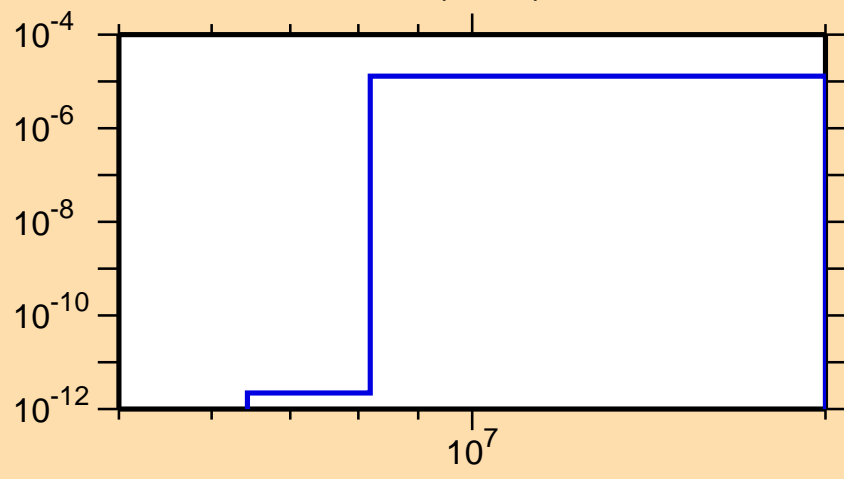
\sigma vs. E for ^{160}\text{Gd}(n,n\alpha)
