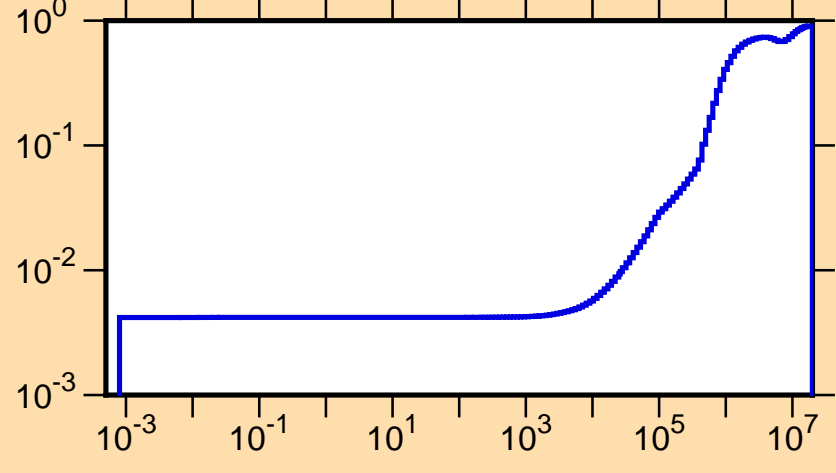
\mu vs. E for ^{161}\text{Gd}(\text{mt251})
