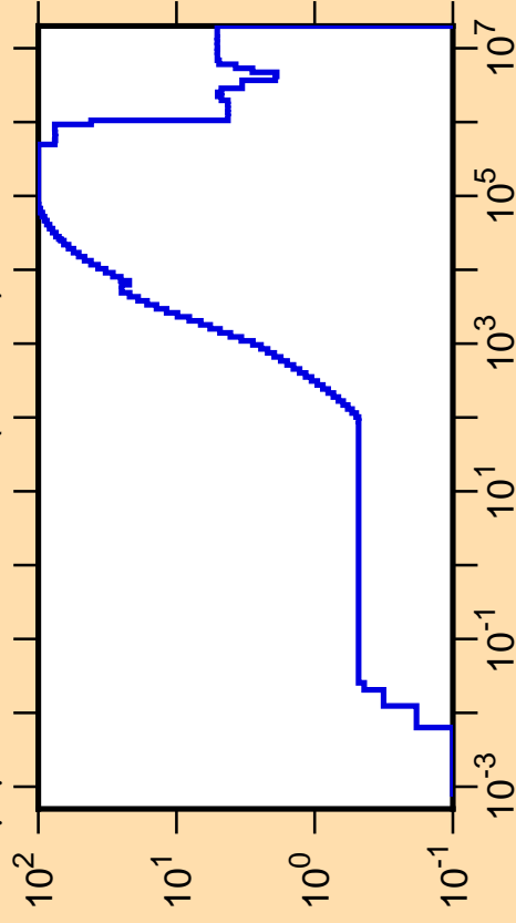
\Delta\mu/\mu vs. E for ^{161}\text{Gd}(\text{mt251})
