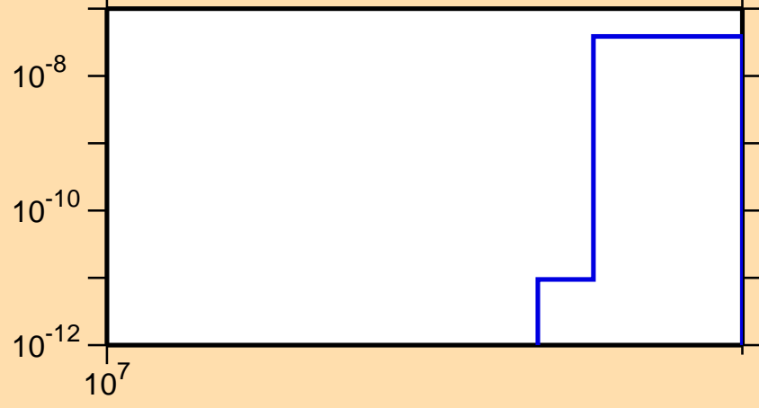
\sigma vs. E for ^{161}\text{Gd}(n,nt)
