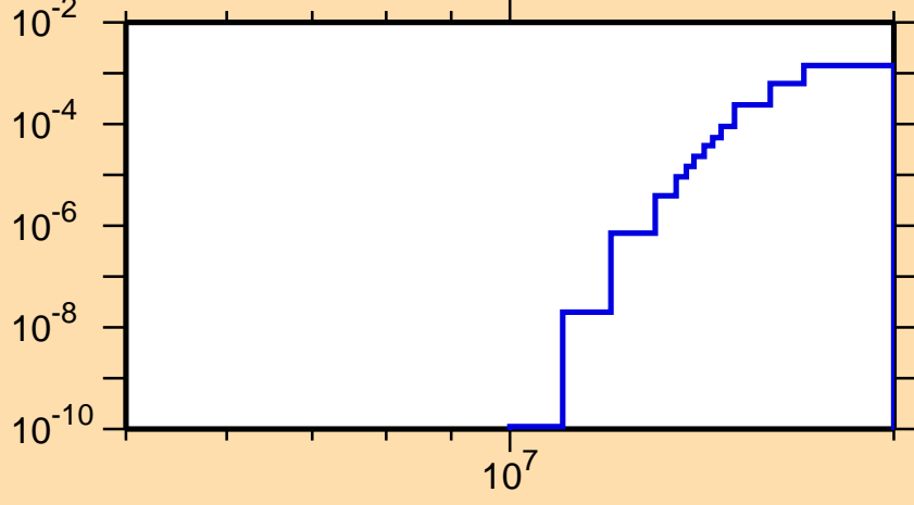
\sigma vs. E for ^{161}\text{Gd}(n,d)
