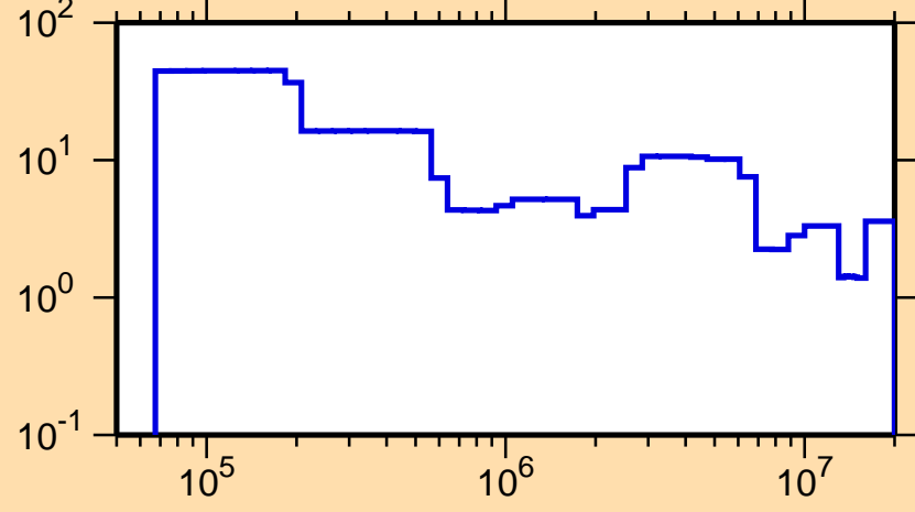
\Delta\sigma/\sigma vs. E for ^{161}\text{Gd}(n,\text{el.})
