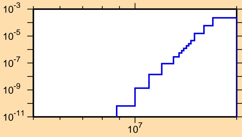
\sigma vs. E for ^{161}\text{Gd}(n,\alpha)
