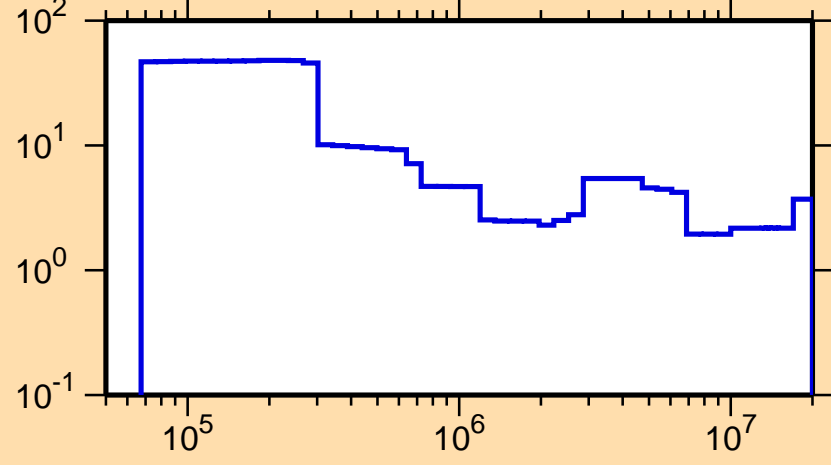
\Delta\sigma/\sigma vs. E for ^{162}\text{Gd}(n,\text{tot.})
