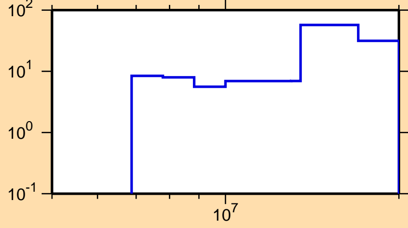
\Delta\sigma/\sigma vs. E for ^{162}\text{Gd}(n,2n)
