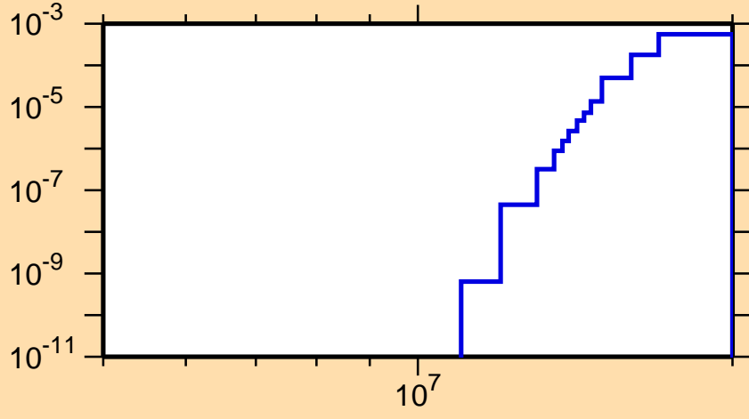
\sigma vs. E for ^{162}\text{Gd}(n,d)
