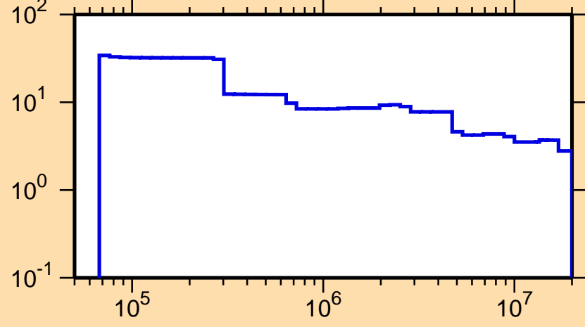
\Delta\sigma/\sigma vs. E for ^{162}\text{Gd}(n,\text{nonel.})
