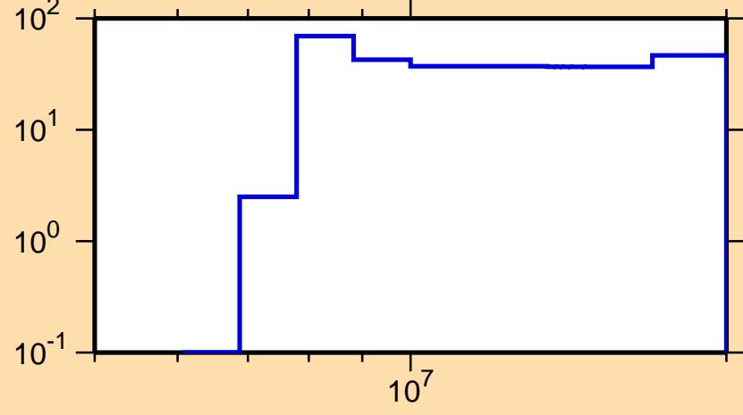
\Delta\sigma/\sigma vs. E for ^{162}\text{Gd}(n,p)
