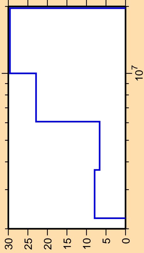
\Delta\sigma/\sigma vs. E for ^{162}\text{Gd}(n,ncont.)
