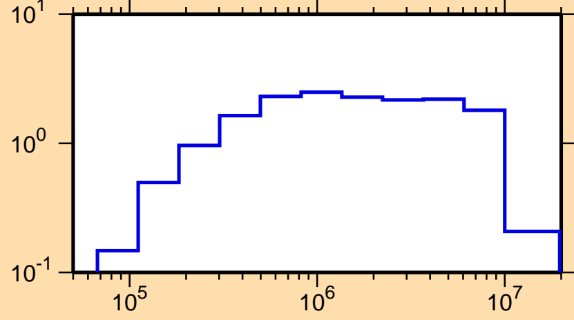
\sigma vs. E for ^{162}\text{Gd}(n,\text{inel.})
