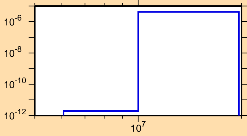
\sigma vs. E for ^{162}\text{Gd}(n,\alpha)
