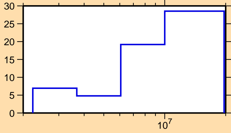
\Delta\sigma/\sigma vs. E for ^{162}\text{Gd}(n,inel.)
